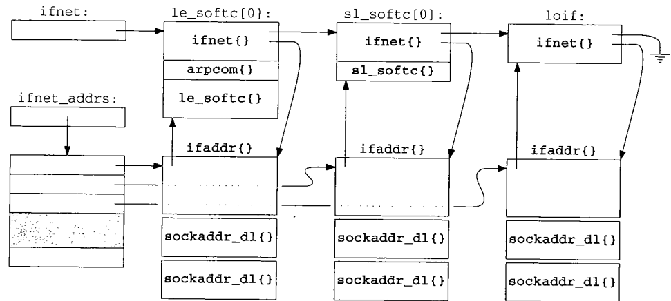
Figure 3.32 ifnet list.
