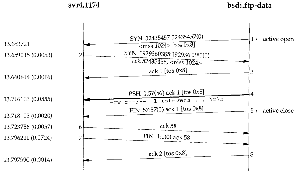
Figure 27.7 Data connection for FTP example.
