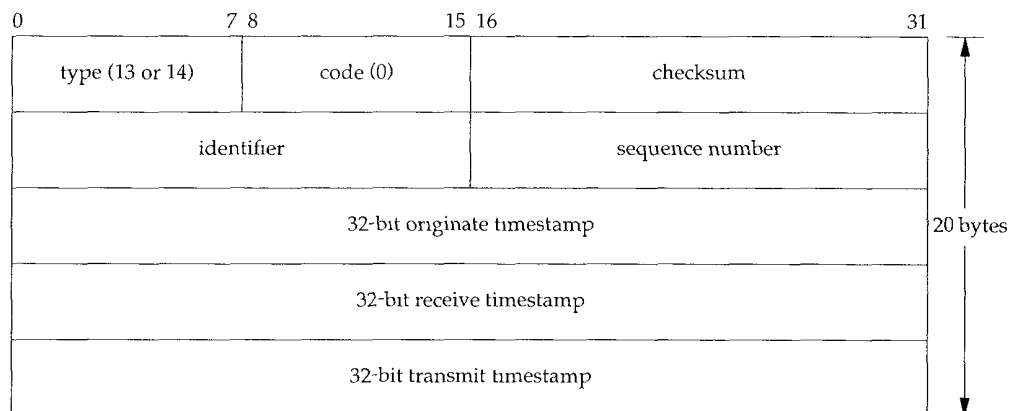
Figure 6.6 ICMP timestamp request and reply messages.
