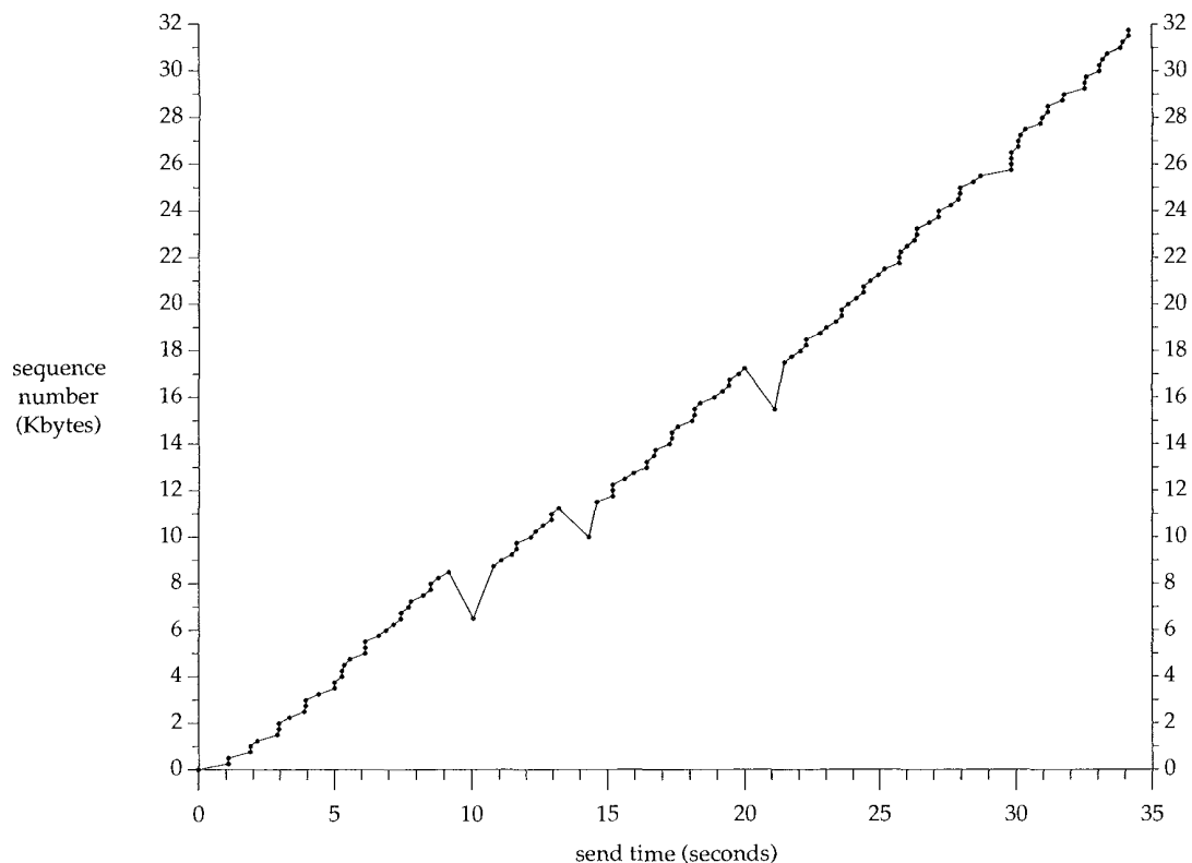
Figure 21.6 Sending of 32768 bytes of data from s11p to vangogh.
