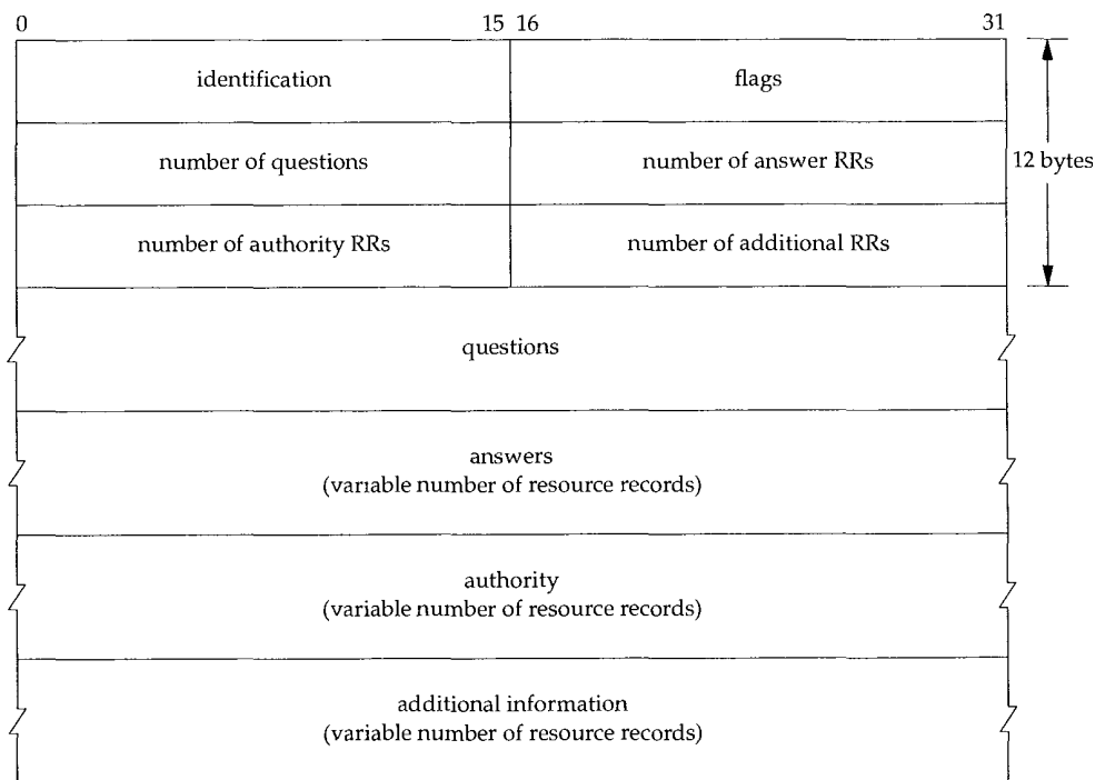
Figure 14.3 General format of DNS queries and responses.
