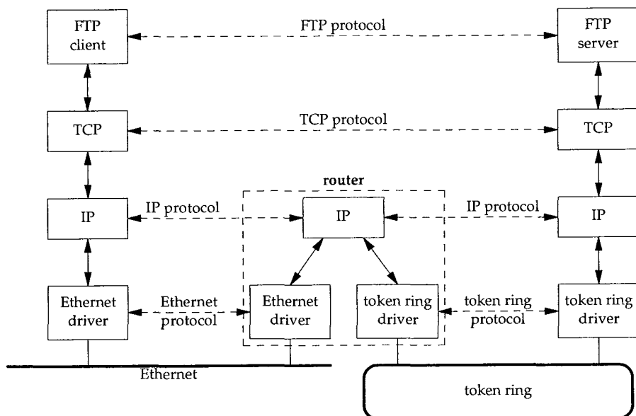
Figure 1.3 Two networks connected with a router.
