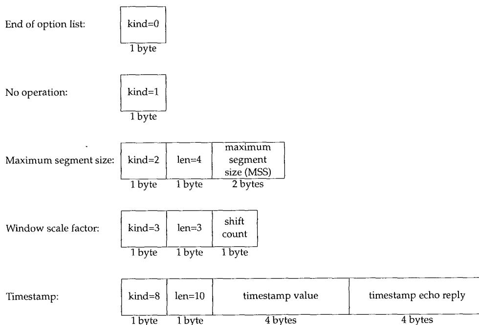
Figure 18.20 TCP options.
