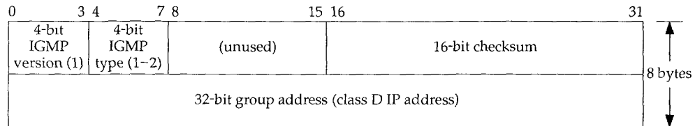
Figure 13.2 Format of fields in IGMP message.
