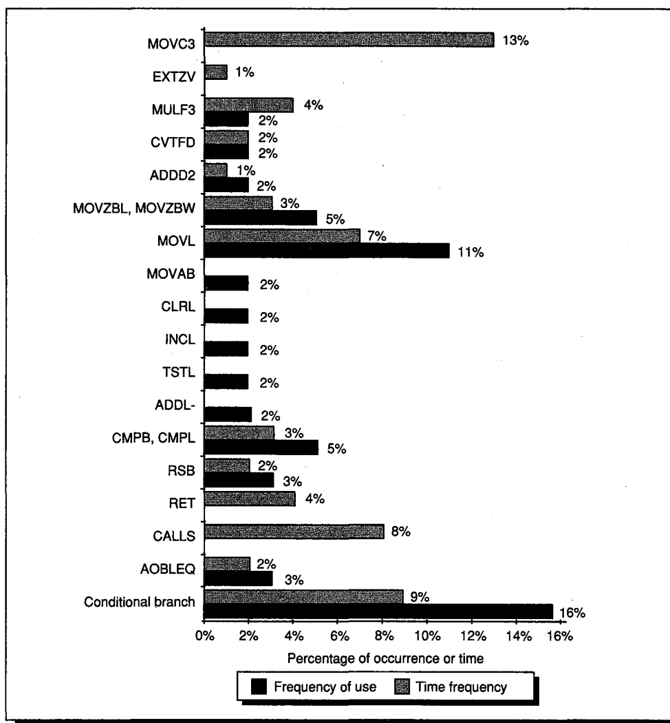
FIGURE D.1 Time and frequency distribution for a multiuser workload on a VAX-11/780 running VMS. This data includes all user instructions that are responsible for more than 1% of either the instruction executions or the execution time. (Two operating system instructions (REI and MTPR), each of which accounts for about 1% of the execution time, are not included.) The absence of an execution-frequency bar or time-frequency bar for an entry (such as MOV3 or TSTL) means that the time frequency or execution-time frequency is below 1% (not that it is 0!). Clark and Levy [1982] commented that the large percentage of time consumed by the MOV3 in the time distribution is somewhat abnormal for a nonbusiness workload and has not been observed in other measurements on the 11/780.
