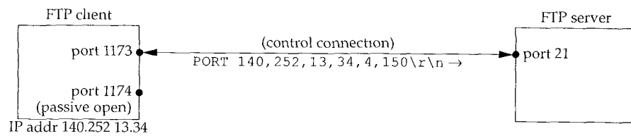
Figure 27.4 PORT command going across FTP control connection.
