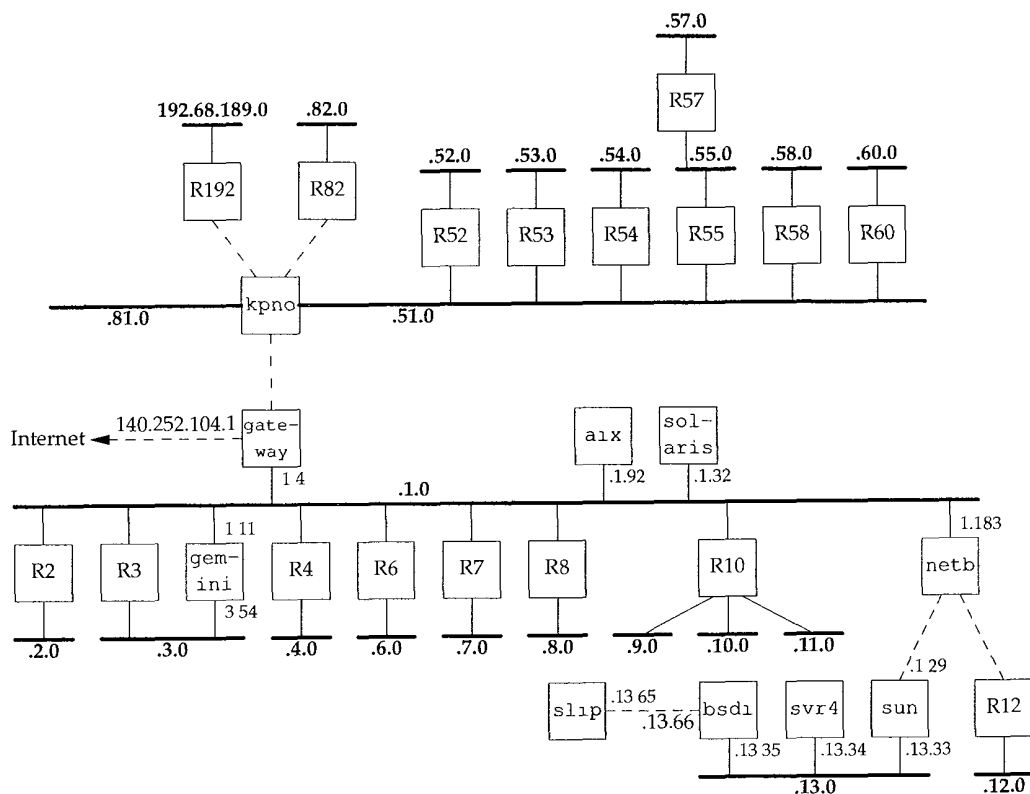
Figure 3.6 Arrangement of most of the noao.edu 140.252 subnets.
