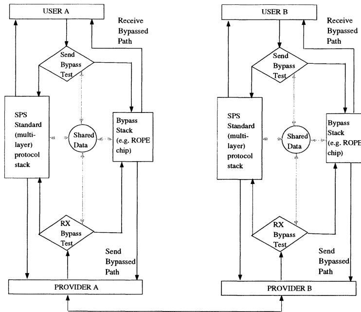
Figure 1 Bypass Architecture
