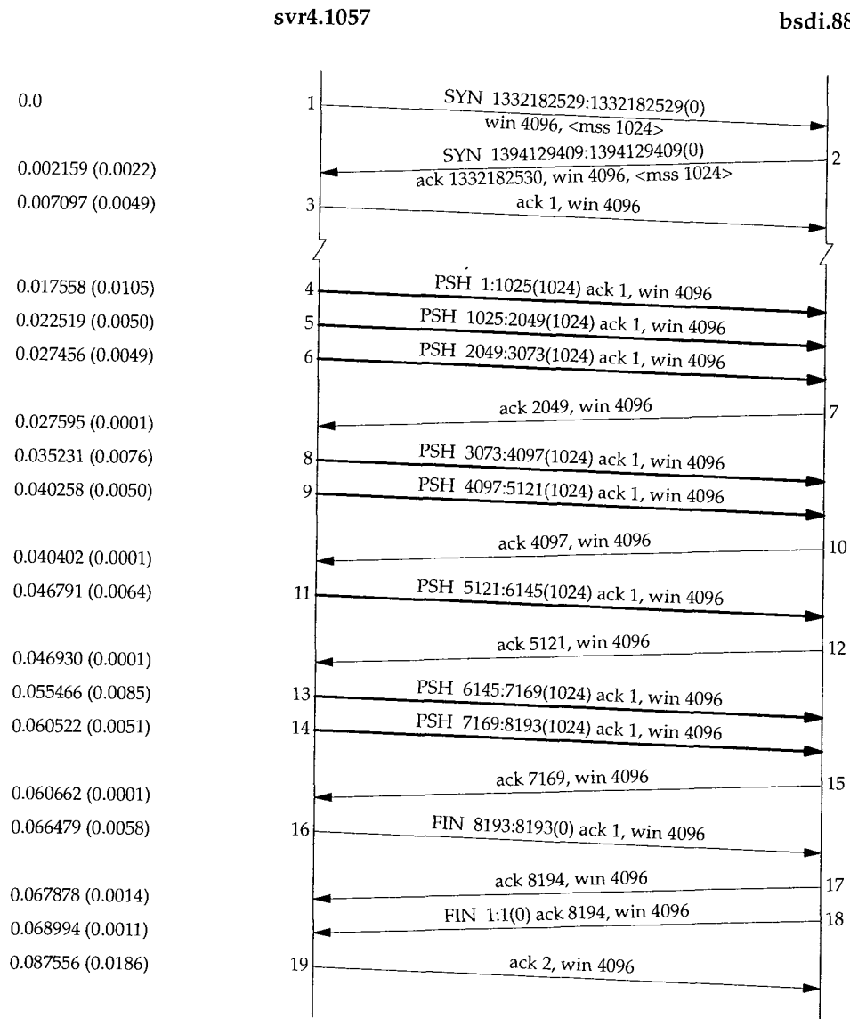
Figure 20.2 Another transfer of 8192 bytes from svr4 to bsd .
