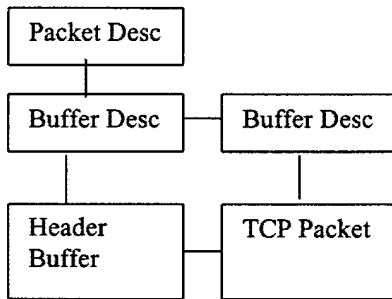
Example of incoming TCP pkt
