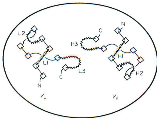
Figure 1. Outline structure of the antigen-binding site. The site is formed by 6 loops of polypeptide ( \blackline ) linked to strands in \beta -sheets ( \square ).
