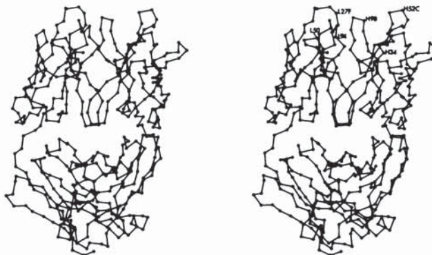
FIG. 4. Stereo view of the C_\alpha skeleton of the J539 Fab structure. Open circles, McPC603 hypervariable residues that were excluded.
