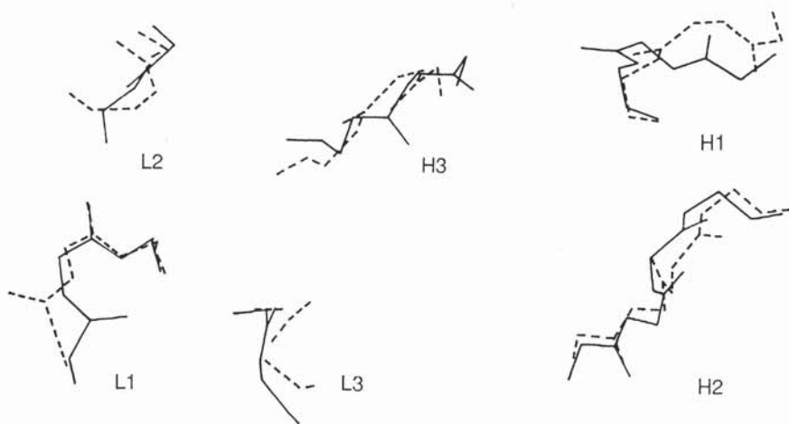
Fig. 2. The main chain atoms of the part of the binding site that makes contact with the antigen (1), in the experimental structure (—) and in the predicted model based on analysis of the known structures (---). The actual relative positions of the regions in the structure are shown from a viewpoint roughly perpendicular to the plane of the antigen-antibody interface.
