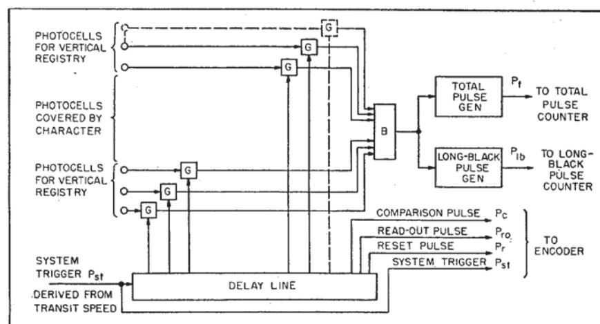
FIG. 3—Scanning station of character reader
