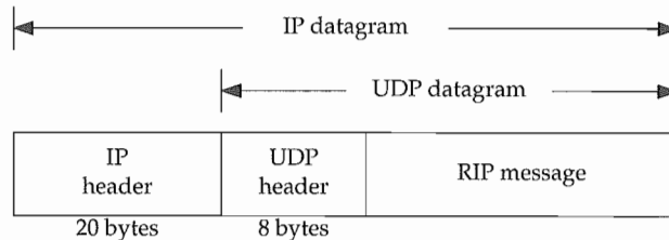
Figure 10.2 RIP message encapsulated within a UDP datagram.
