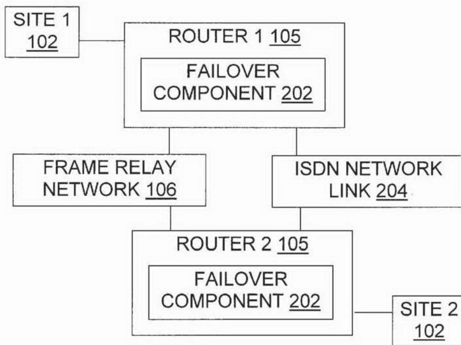
(PRIOR ART)
