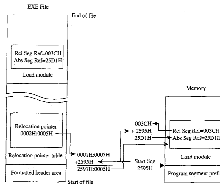
Figure 4-6 The EXE file relocation procedure
