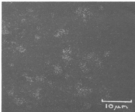
Fig. 5. Scanning electron micrograph of the system in Fig. 4 under EDAX.
