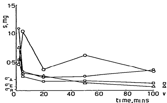
Fig. 6. Plot of standard deviation of sulphaphenazole content of 20 x 200-mg samples vs. time for mixing of 2% sulphaphenazole with Dipac — Unsifted, \circ ; 180 - 250- \mu\text{m} , \triangle ; 250 - 355- \mu\text{m} , \square ; 355 - 500- \mu\text{m} , \diamond .
