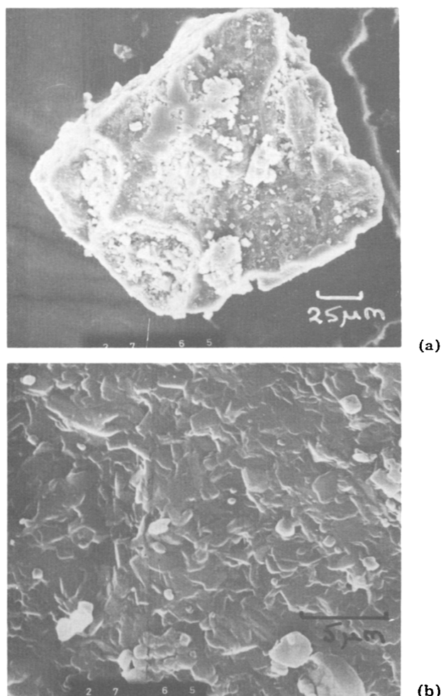
Fig. 7. Scanning electron micrographs of a Dipac particle (180 - 250- \mu\text{m} sieve fraction).
