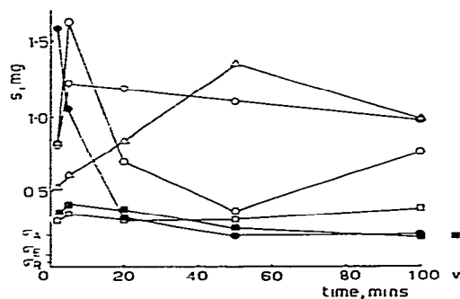
Fig. 1. Plot of standard deviation of sulphaphenazole content of 20 x 200-mg samples vs. time for mixing of 2% sulphaphenazole with Celutab — Unsifted, \circ ; 180 - 250- \mu\text{m} , \square ; 250 - 355- \mu\text{m} , \triangle ; 355 - 500- \mu\text{m} , \diamond ; 500 - 710- \mu\text{m} , \bullet ; 710 - 1000 \mu\text{m} , \blacksquare . \sigma_R is the theoretical standard deviation of the fully randomised mix neglecting standard deviation of the sampling and analytical procedure, \sigma_S . \sigma_E is equal to the sum of \sigma_R and \sigma_S . \sigma_A is a typical manufacturers mixing specification as given by eqn. (4).
