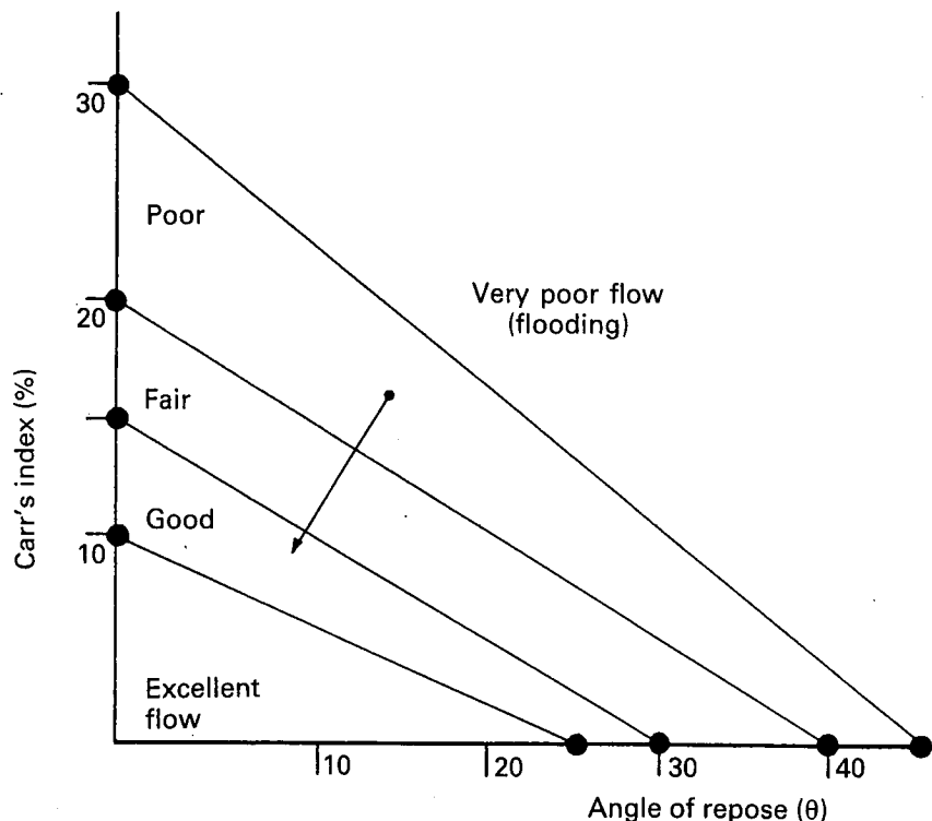
Fig. 13.6 Relationship between the angle of repose and Carr's index of a powder and its flow characteristics
