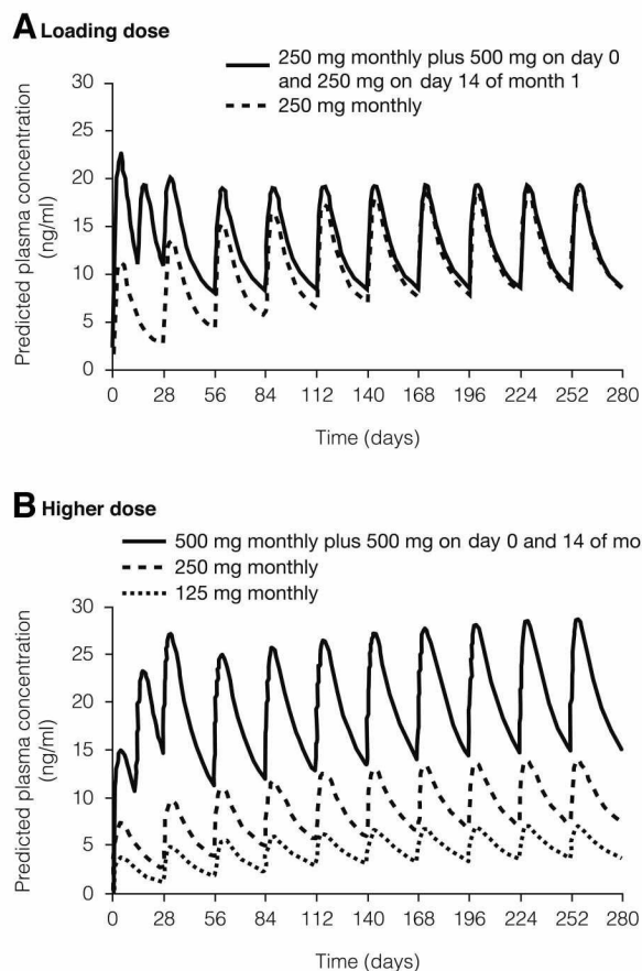
Figure 3. Pharmacokinetic models for loading-dose (A) and high-dose (B) fulvestrant regimens.
