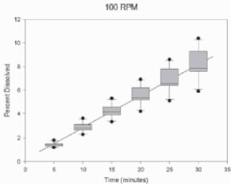
Figure 7. Box plot of paddle apparatus at 100 rpm
