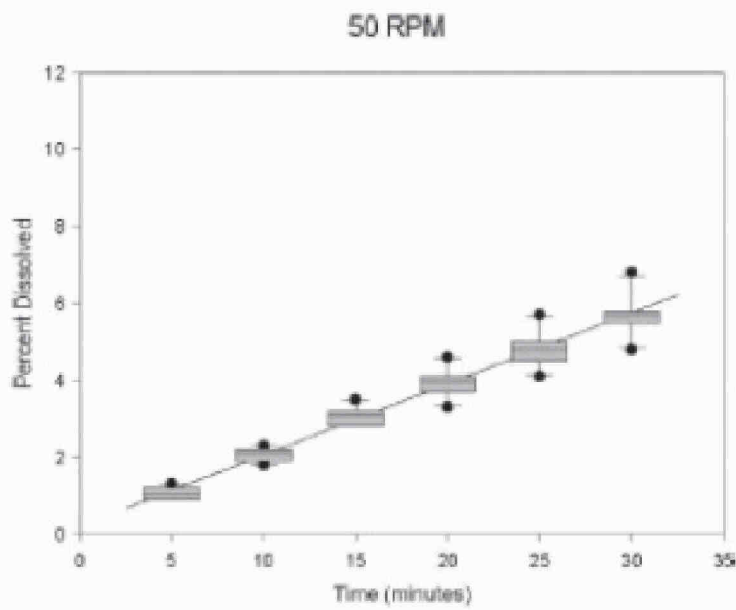
Figure 6. Box Plot of paddle apparatus at 50 rpm
