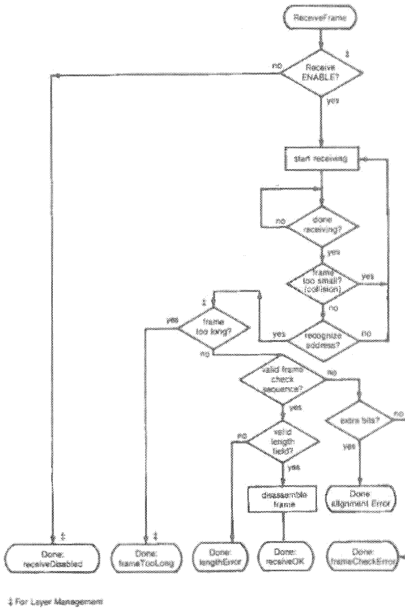
(b) ReceiveFrame
