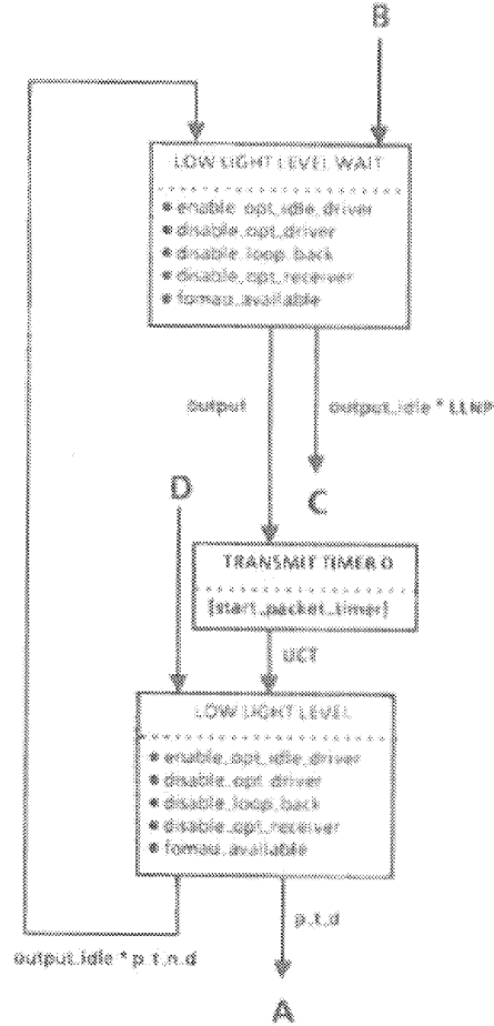
Fig 9-10 Low Light Level Detection Function State Diagram
