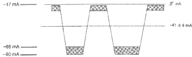
Fig 8-5 Recommended Driver Current Signal Levels
