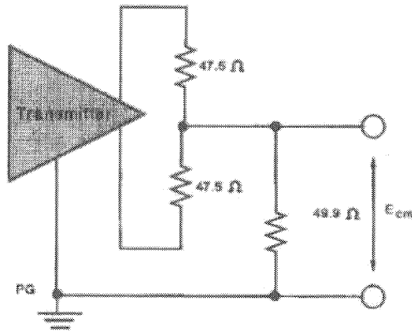
Fig 14-14 Common-Mode Output Voltage Test Circuit
