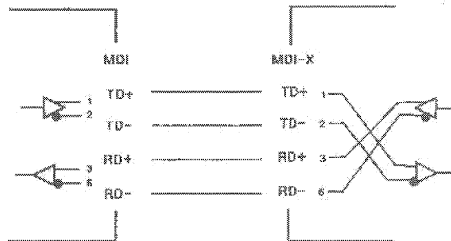
(b) MAU-Embedded Crossover Function
