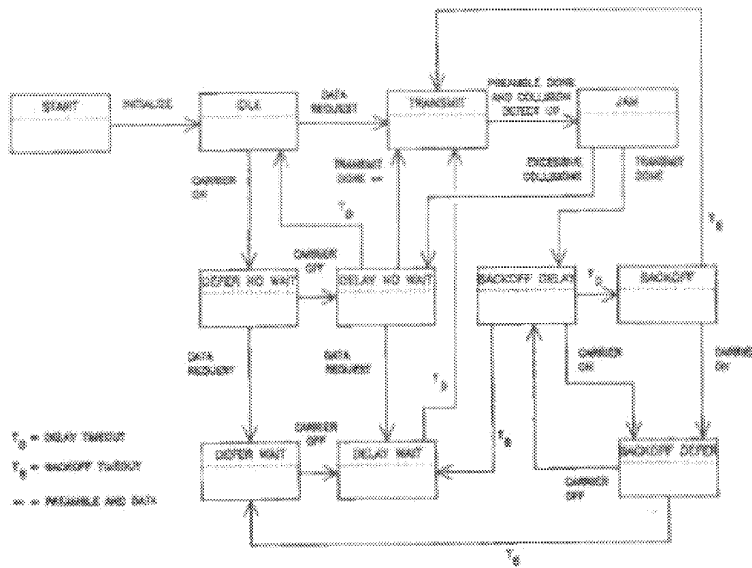
Fig B1 Transmit Component State Diagram
