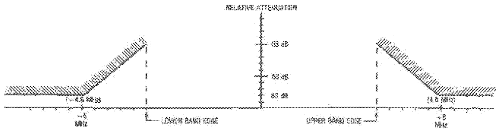
Fig 11-7 Spectrum Mask for RF Data Signal
