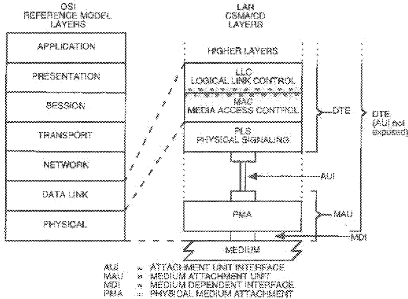
Fig 2-1 Service Specification Relation to the LAN Model
