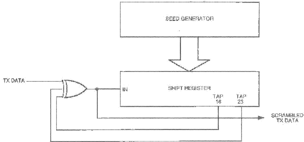
Fig 11-10 Scrambler
