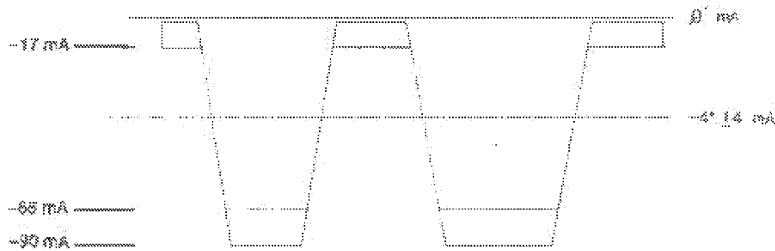
Fig 10-4 Driver Current Signal Levels
