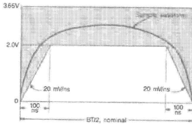
Fig 12-19 Differential Output Voltage, Nominal Duration BT/2
