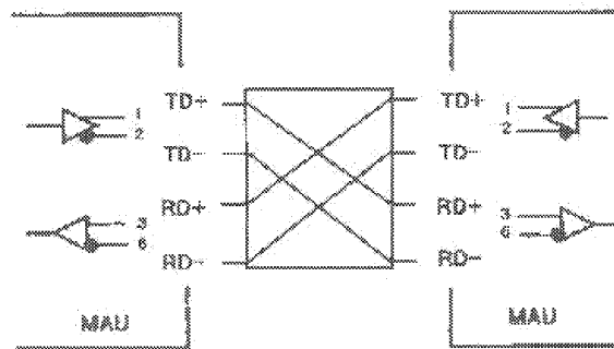
(a) External Crossover Function
