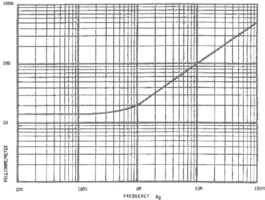
Fig 10-6 Maximum Coaxial Cable Transfer Impedance
