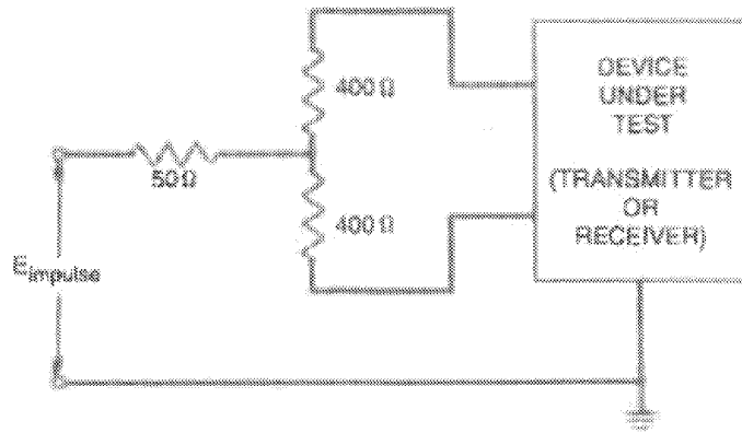
Fig 12-27 Common-Mode Impulse Test
