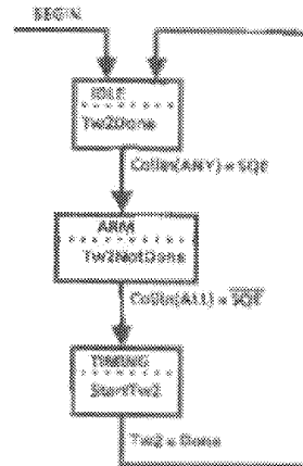
Fig 9-4 Tw2 State Diagram
