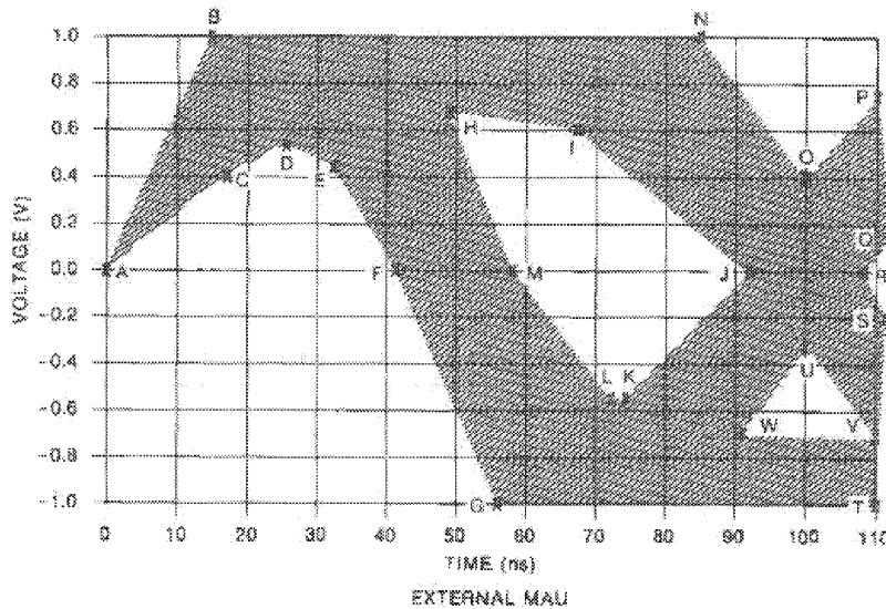
Fig 14-9 Voltage Template
