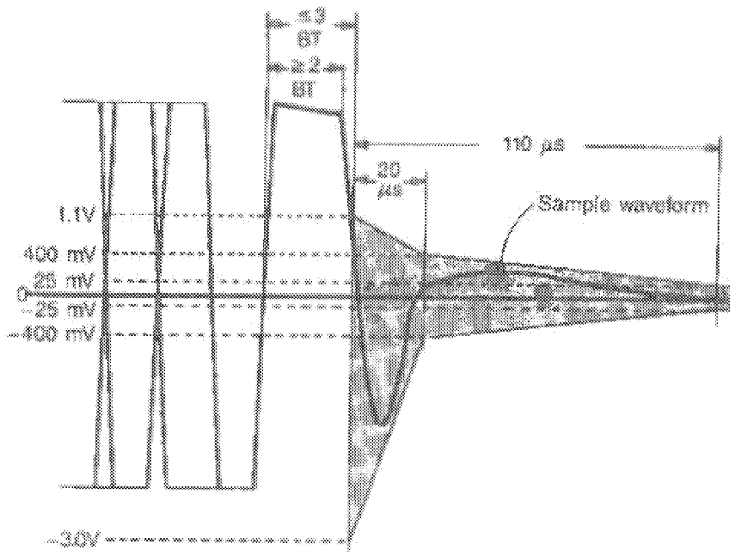
Fig 12-21 Transmitter Waveform for Idle
