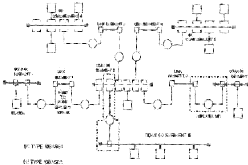
Fig 10-11 An Example of a Large Hybrid System
