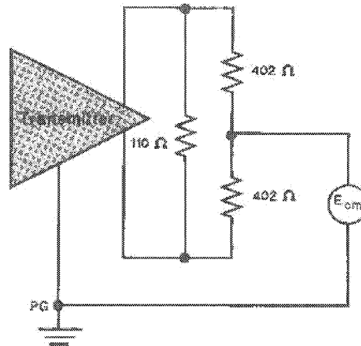
Fig 14-15 Transmitter Fault Tolerance Test Circuit
