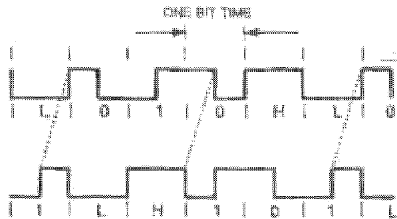
Fig 12-11 Examples of Collision Presence Waveforms
