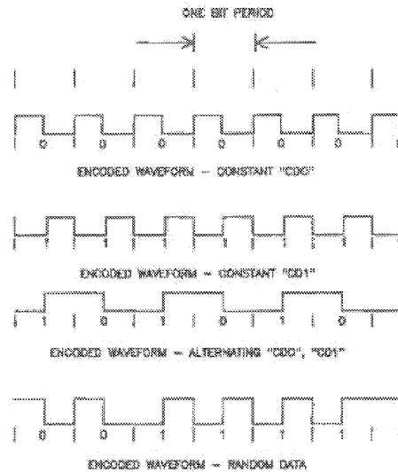
Fig 7-10 Examples of Manchester Waveforms
