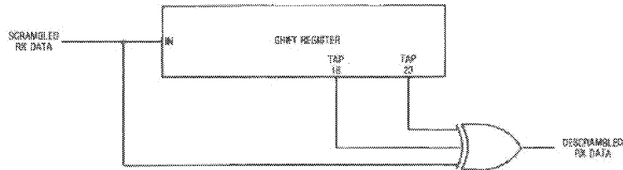
Fig 11-12 Descrambler
