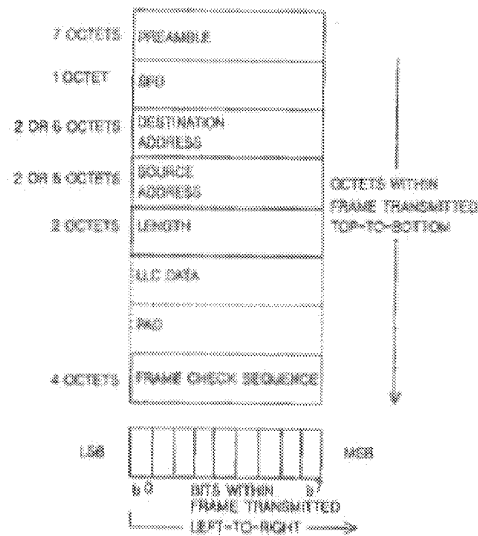
Fig 3-1 MAC Frame Format
