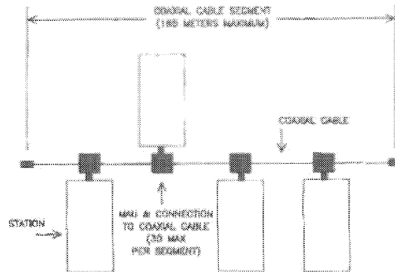
Fig 10-9 The Minimum System Configuration
