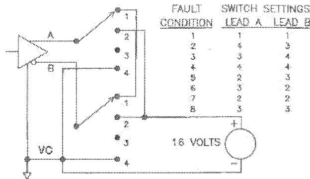
Fig 7-14 Driver Fault Conditions
