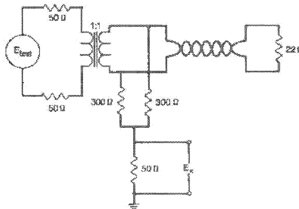
Fig 12-32 Cable Balance Test
