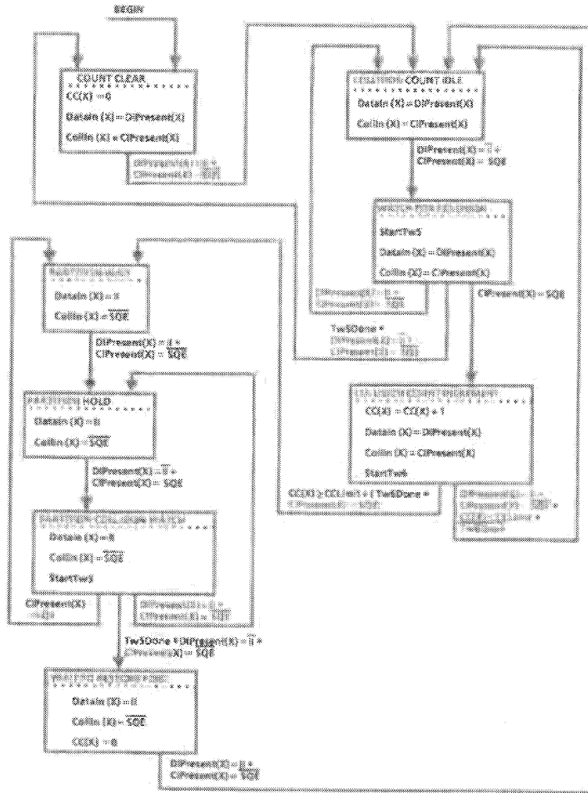
Fig 9-8 Partitioning State Diagram for Port X
