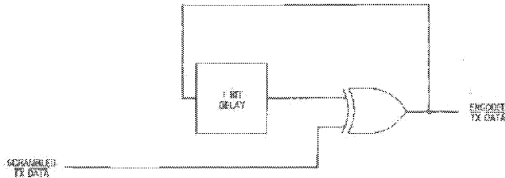
Fig 11-11 Differential Encoder
