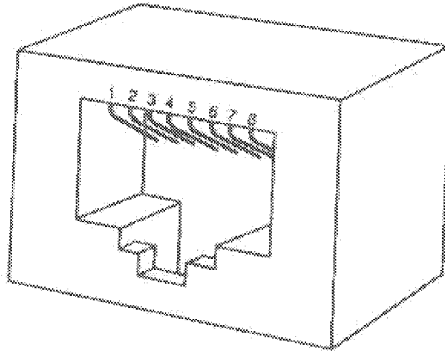
Fig 12-30 DTE and Hub Connector
