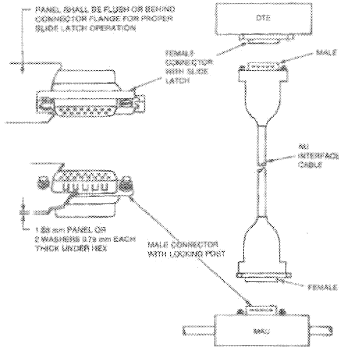
Fig 7-20 Connector Hardware and AUI Cable Configuration
