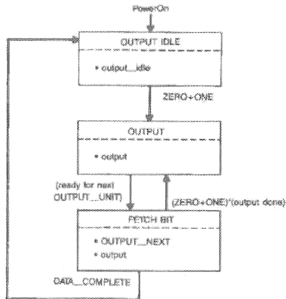
Fig 12-6 DTE PLS Output Function
