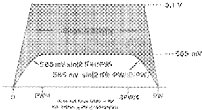
Fig 14-17 Receiver Differential Input Voltage—Wide Pulse
