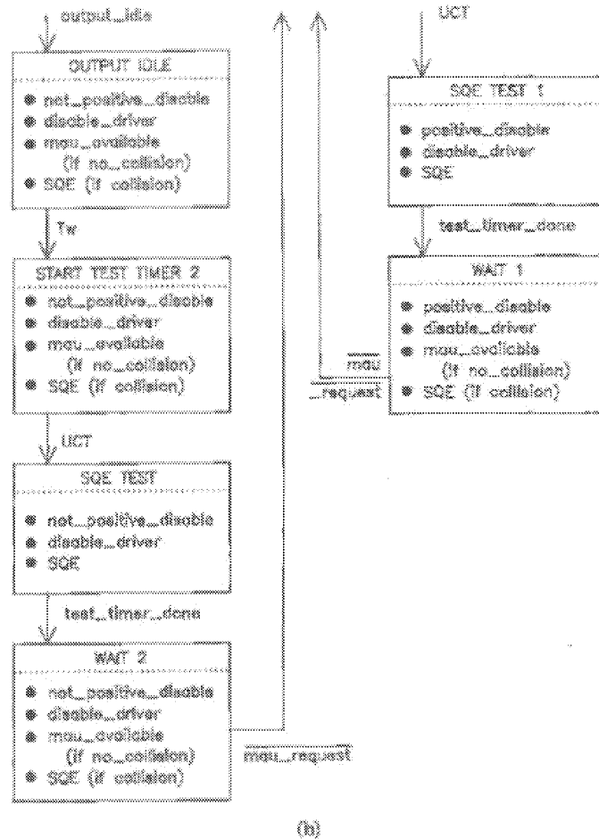
Fig 7-9 Interface Function for MAU with Conditioning
