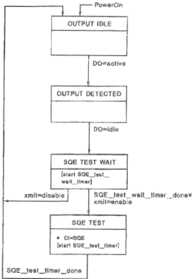
Fig 14-4 signal_quality_error Message Test Function State Diagram
