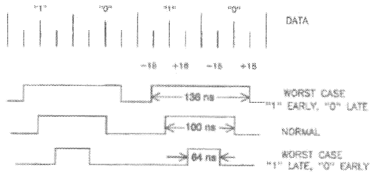
Fig A3 Worst-Case Signal Waveform Variations
