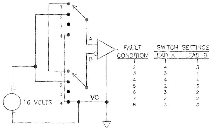
Fig 7-16 Receiver Fault Conditions
