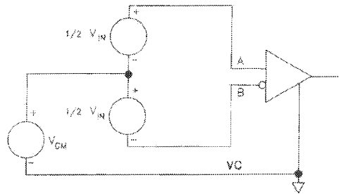
Fig 7-15 Common-Mode Input Test
