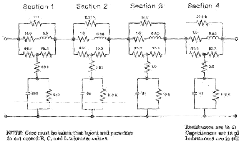
Fig 14-7 Twisted-Pair Model
