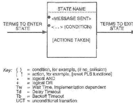
Fig 1-2 State Diagram Notation Example
