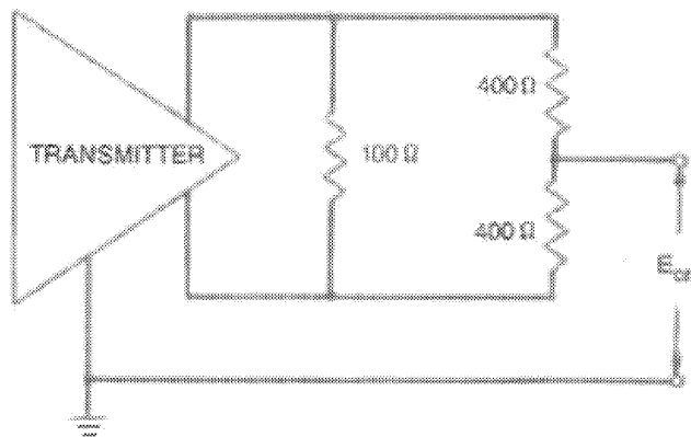
Fig 12-26 Transmitter Common-Mode Tolerance
