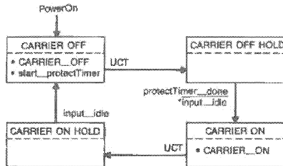
Fig 12-9 DTE PLS Carrier Sense Function
