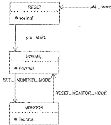
Fig 7-4 PLS Mode Function
