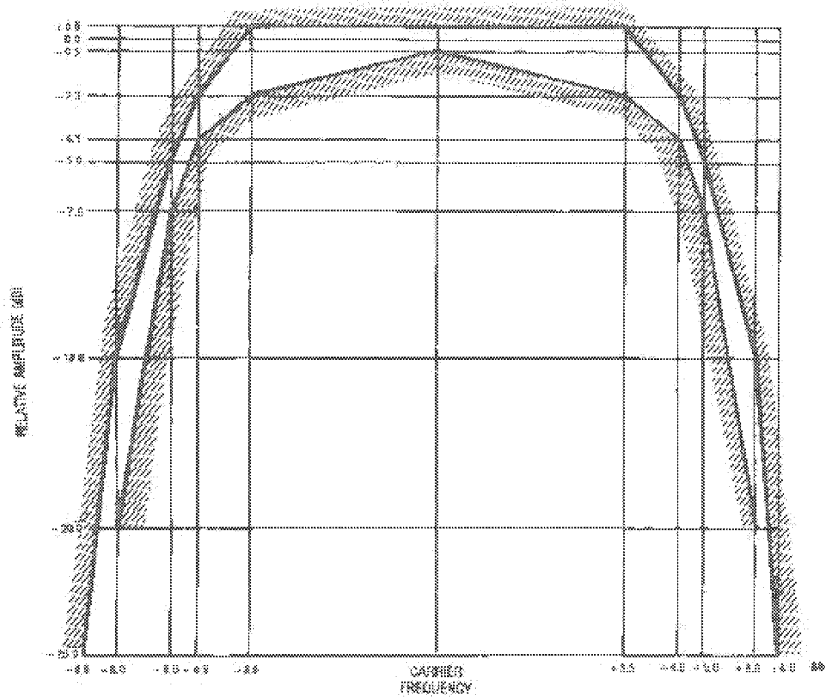
Fig 11-7 Spectrum Mask for RF Data Signal
