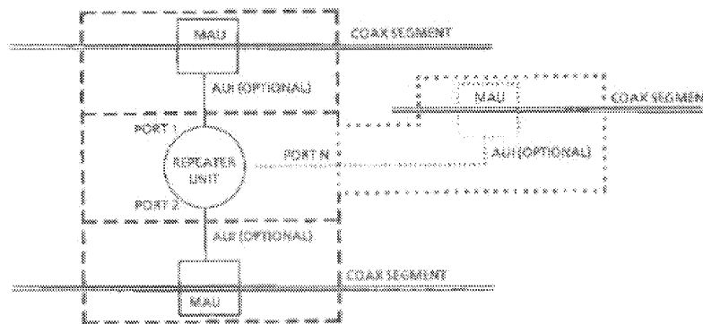
Fig 9-1 Repeater Set, Coax-to-Coax Configuration
