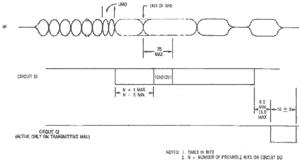
Fig 11-13 No Collision Timing Diagram (Coax to AUI)
