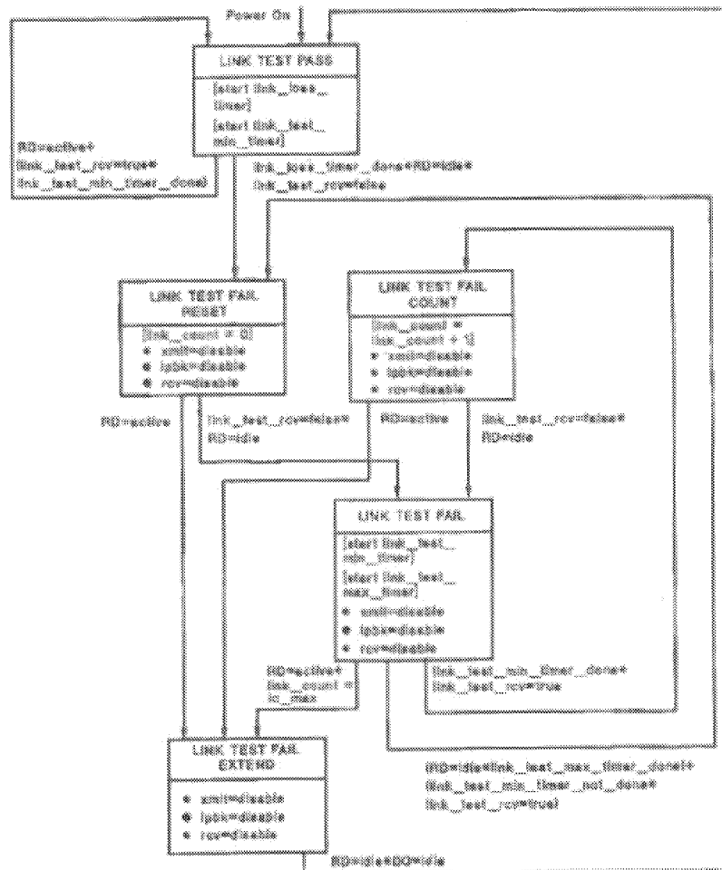
Fig 14-6 Link Integrity Test Function State Diagram
