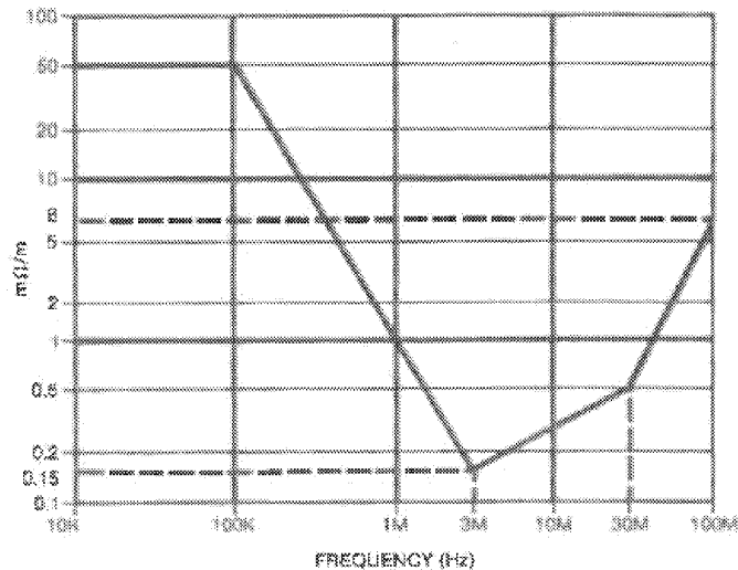
Fig 8-7 Maximum Coaxial Cable Transfer Impedance
