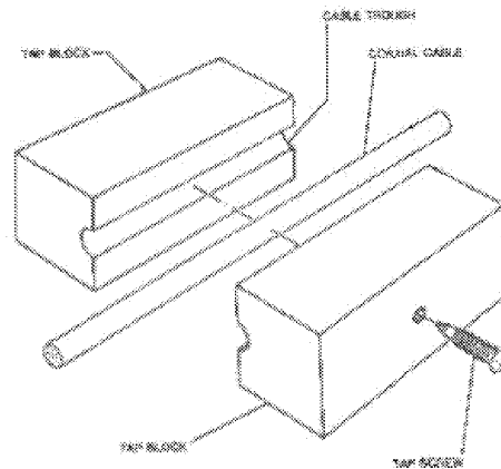
Fig 8-8 Coaxial Tap Connector Configuration Concepts
