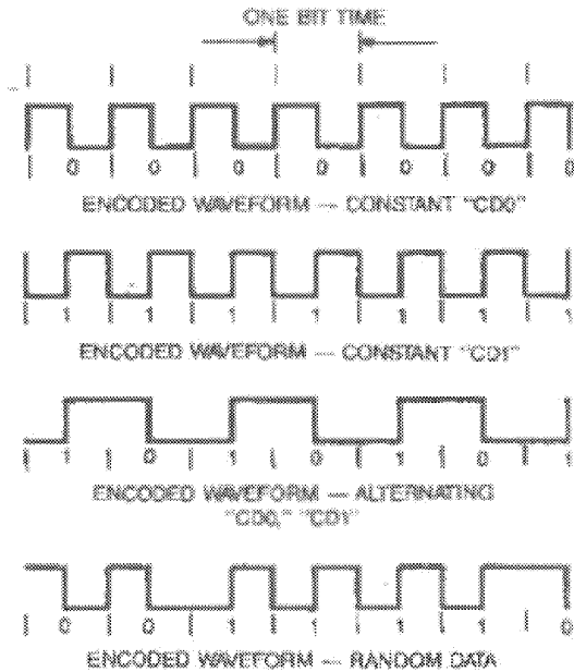
Fig 12-10 Examples of Manchester Waveforms
