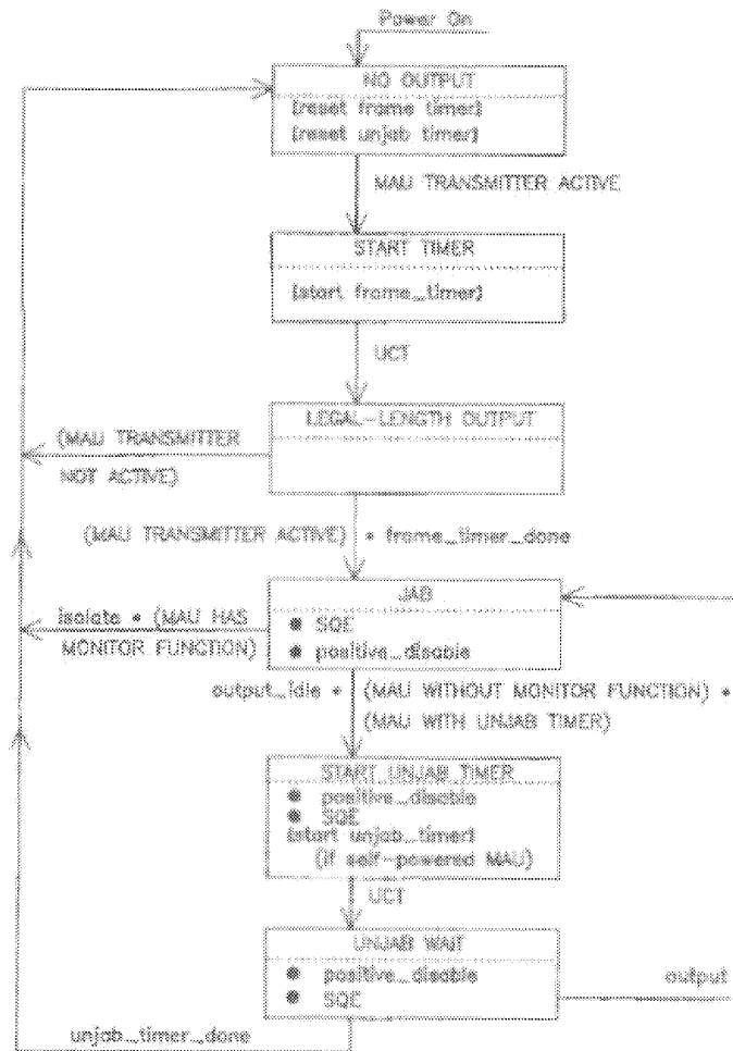
Fig 8-4 Jabber Function
