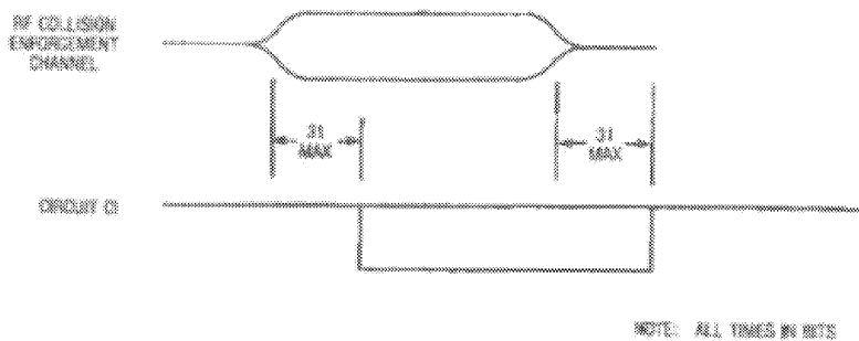
Fig 11-15 Collision Timing Diagram (Coaxial Cable Interface to AUI Circuit CI)
