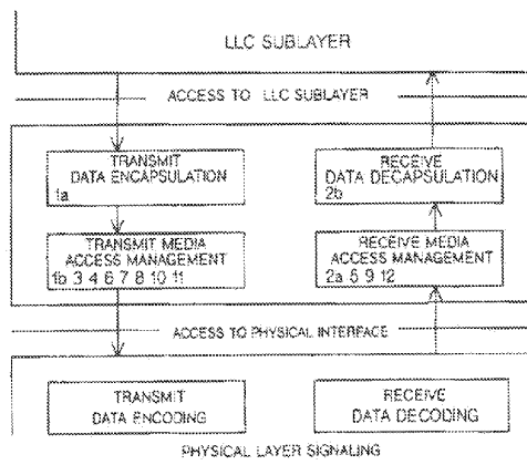
Fig 4-2 CSMA/CD Media Access Control Functions
