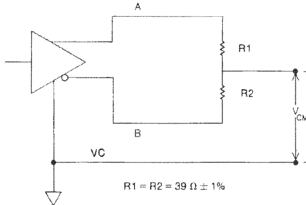
Fig 7-13 Common-Mode Output Voltage
