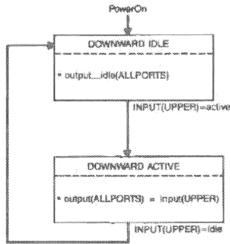
Fig 12-15 Hub PLS Downward Transfer Function
