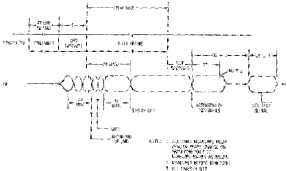
Fig 11-4 Packet Format and Timing Diagram (AUI to Coaxial Cable Interface)
