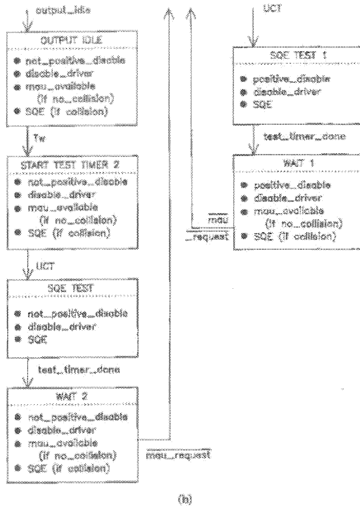
Fig 7-9 Interface Function for MAU with Conditioning
