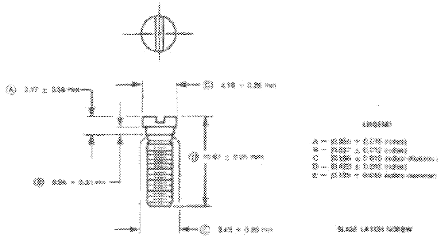
Fig 7-19 Connector Locking Posts
