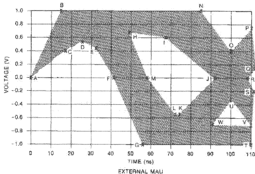
Fig 14-9 Voltage Template
