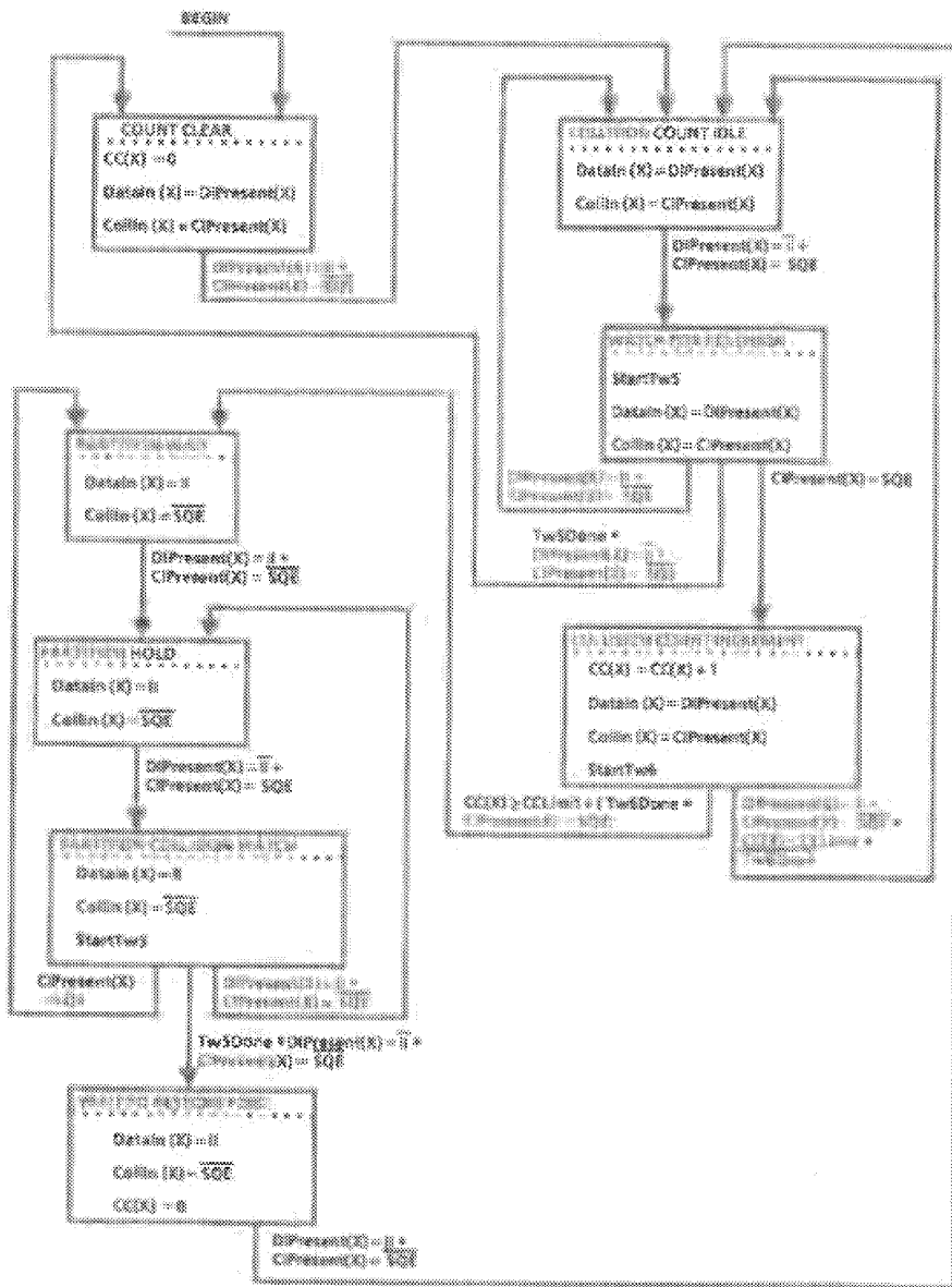
Fig 9-8 Partitioning State Diagram for Port X
