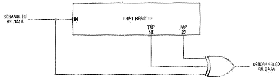
Fig 11-12 Descrambler
