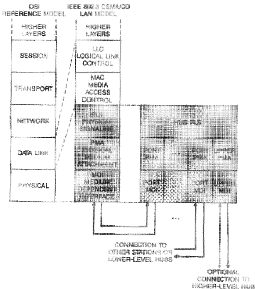
Fig 12-1 IEEE Relationship to the ISO Open Systems Interconnection (OSI) Reference Model and the IEEE 802.3 CSMA/CD LAN Model
