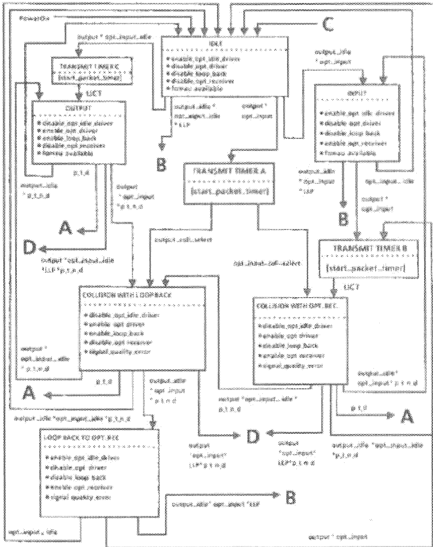
Fig 9-8 FOMA Transmitt, Receive, and Collision Functions State Diagram
