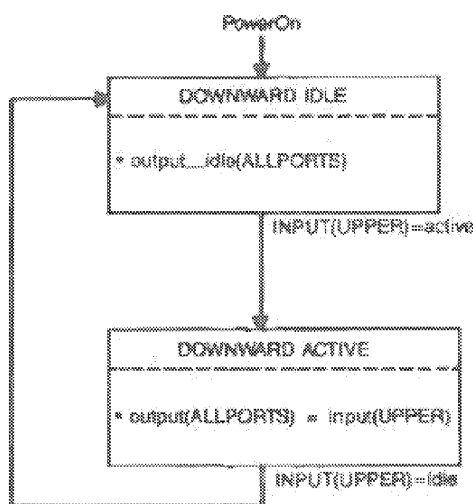
Fig 12-15 Hub PLS Downward Transfer Function
