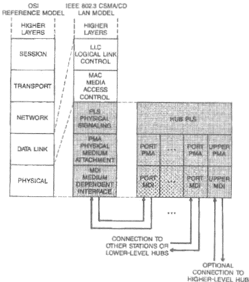
Fig 12-1 IEEE Relationship to the ISO Open Systems Interconnection (OSI) Reference Model and the IEEE 802.3 CSMA/CD LAN Model
