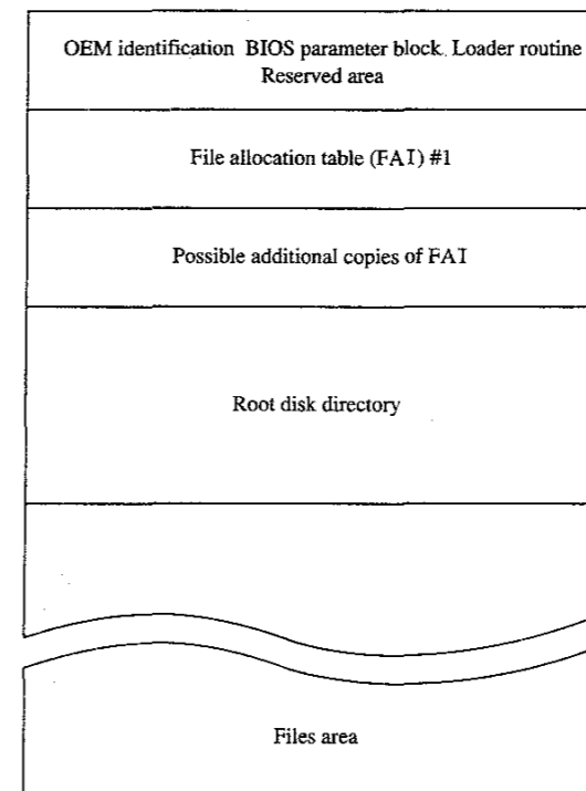
Figure 3-5 The MS-DOS file system
