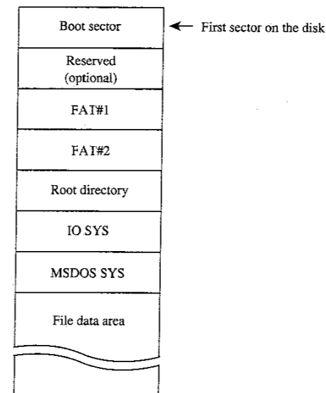
Figure 2-4 Boot-disk configuration
