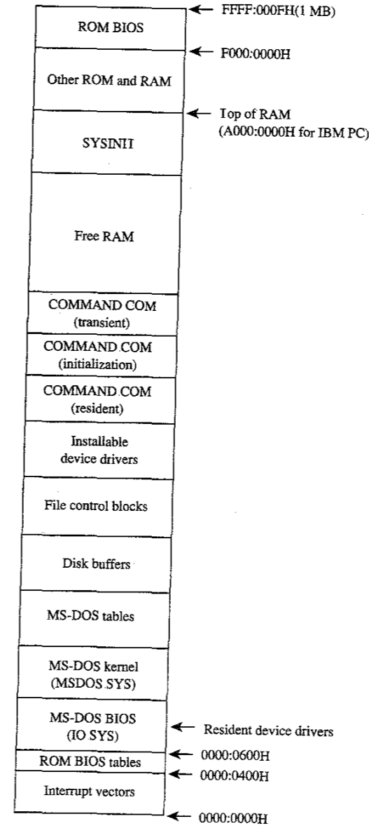
Figure 2-8 COMMAND.COM loaded.
