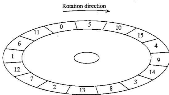
Figure 3-3 A 3:1 interleave
