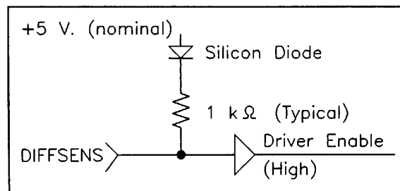
Figure 11 - Termination for differential devices
