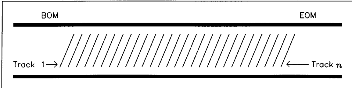
Figure 22 - Helical scan recording example
