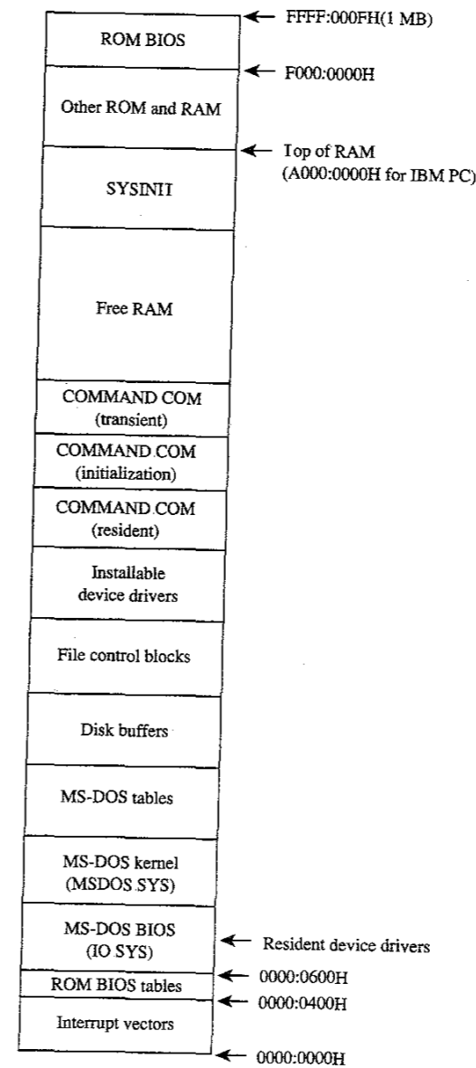
Figure 2-8 COMMAND.COM loaded.
