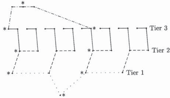
Figure 2.5: Parity-check tree
