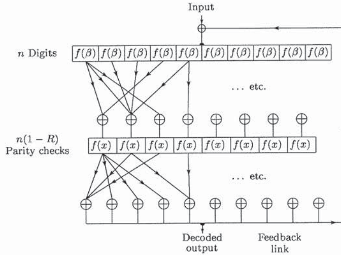
Figure 4.2: Decoding apparatus
