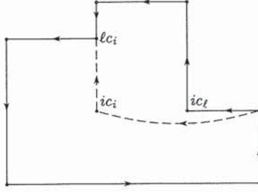
Figure C.7: Case 2: Closed path through \ell c_i and i c_\ell .
