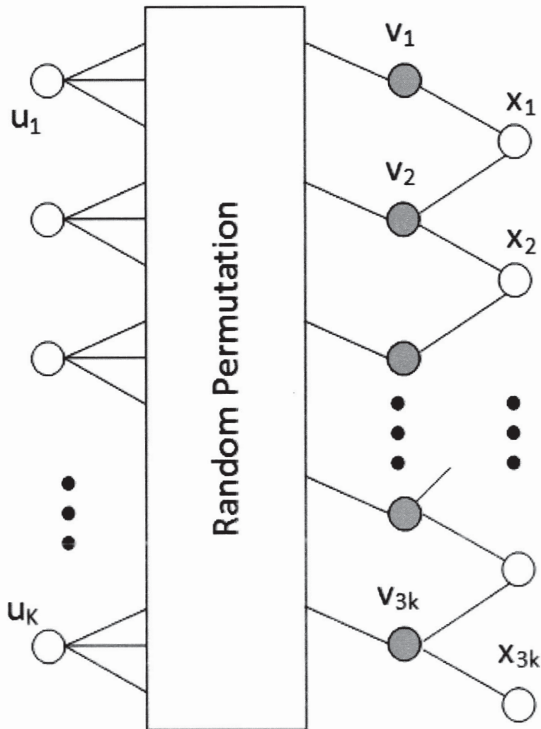
Tanner graph for Divsalar with all information bits having degree 3
