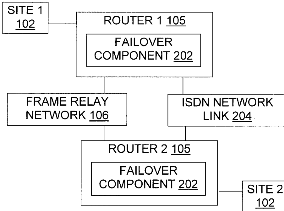
(PRIOR ART)
