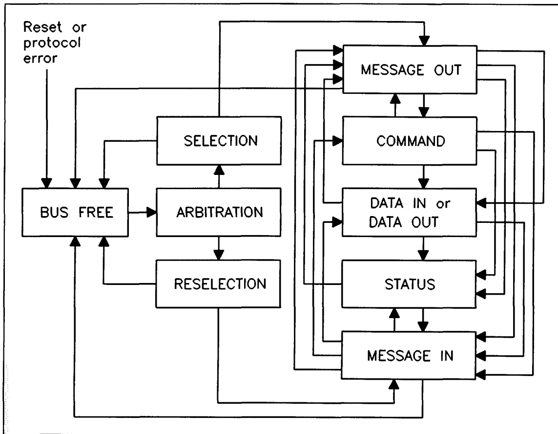
Figure 16 - Phase sequences
