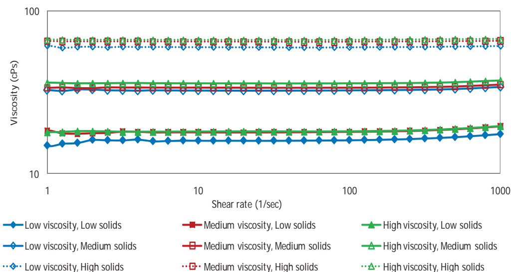
Figure 1. Viscosity of Coating Solutions
