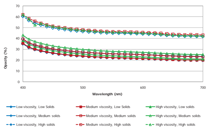
Figure 4. Opacity of Semipermeable Membranes
