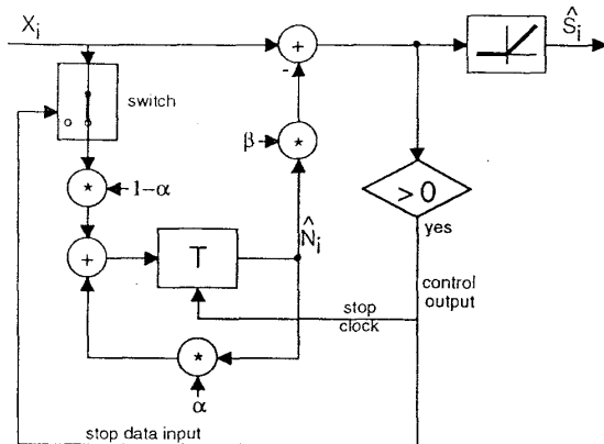
Fig. 1. Simple noise reduction scheme in one subband
