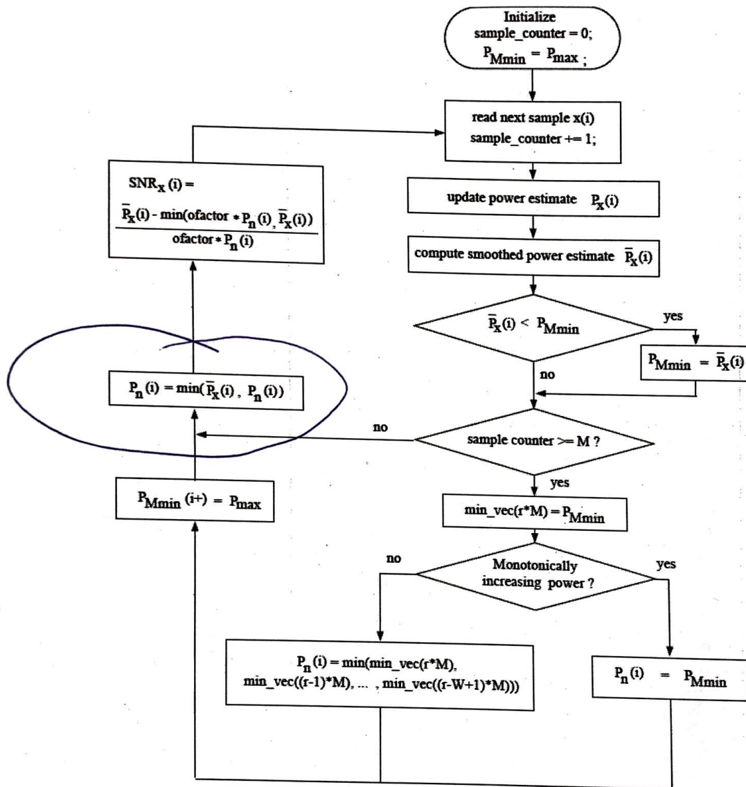
Figure 2: Flowchart of the SNR estimation algorithm
