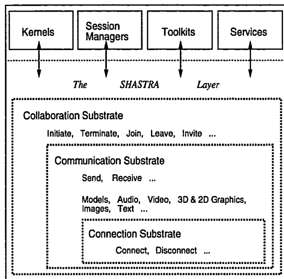
Figure 4.1 The Shastra Layer
