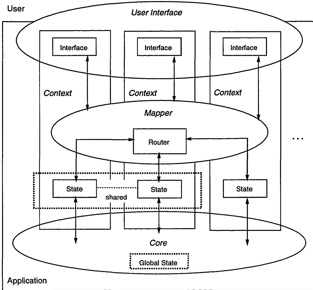
Figure 2.1 Structural Application Model
