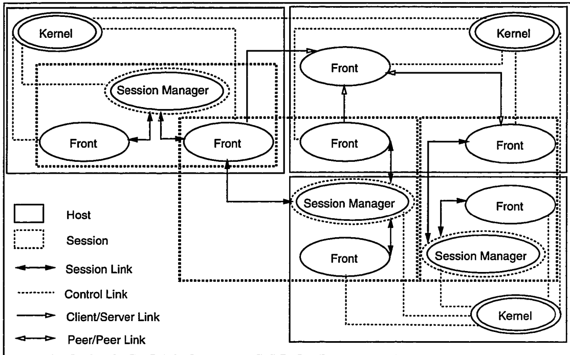
Figure 3.3 Information Flow in the Shastra Environment
