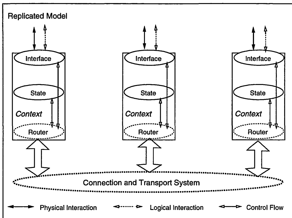
Figure 2.6 Replicated Collaboration Model
