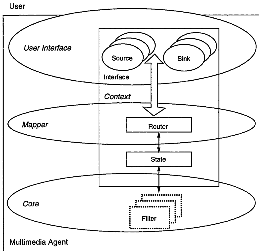
Figure 2.3 Multimedia Application Model
