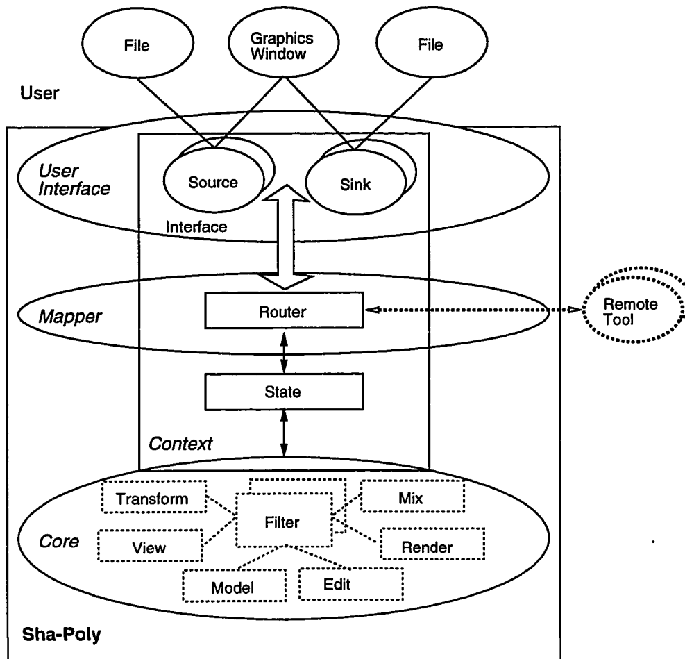
Figure A.3 High Level Architecture of Sha-Poly
