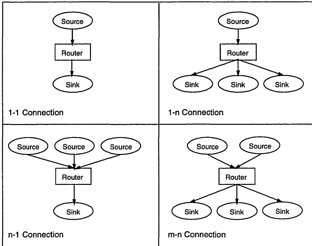
Figure 2.4 Distributed Multimedia Model
