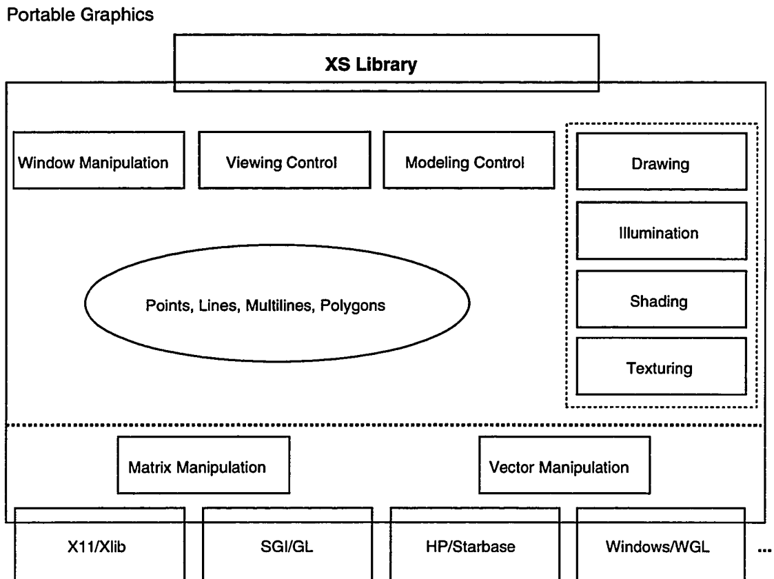
Figure 3.2 High Level Architecture of XS
