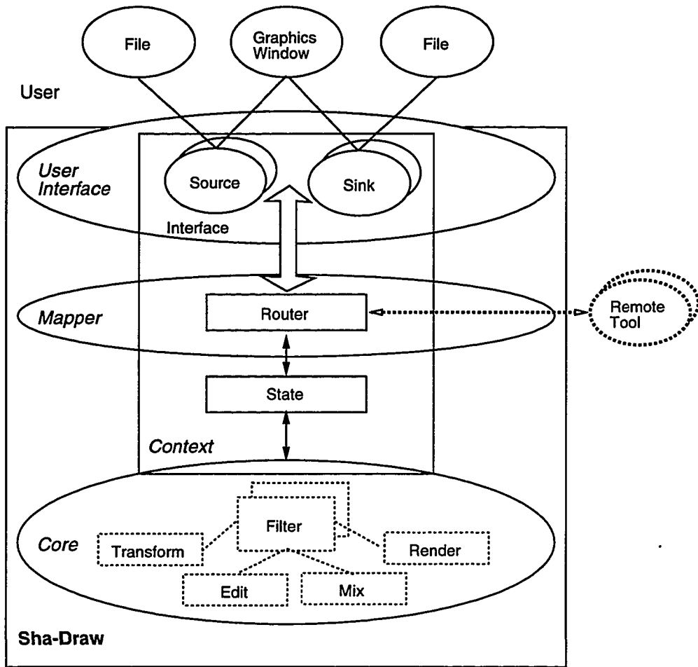
Figure A.2 High Level Architecture of Sha-Draw
