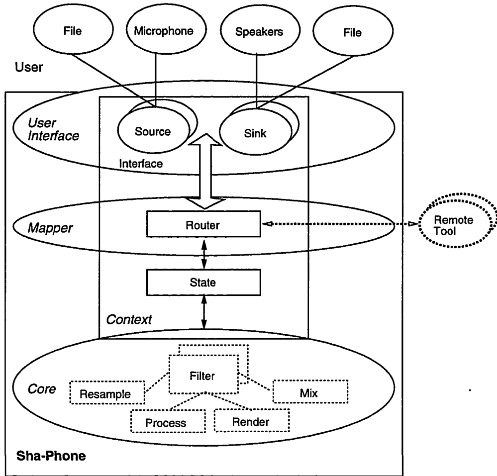
Figure B.4 High Level Architecture of Sha-Phone
