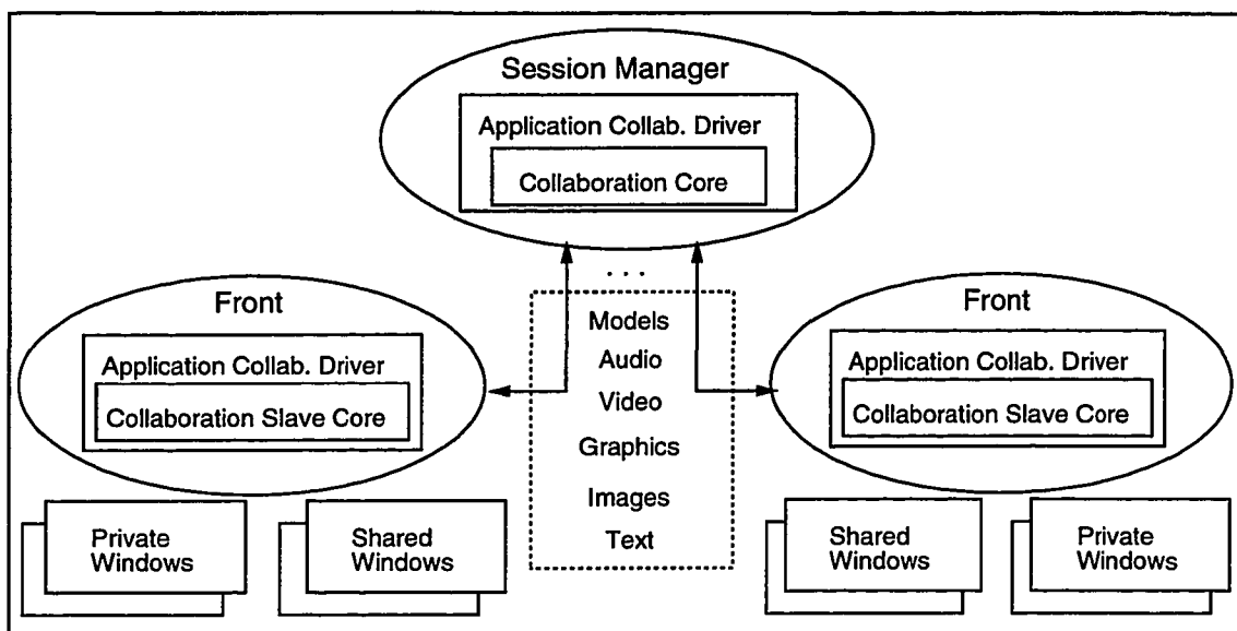
Figure 3.5 Architecture of a Collaborative Session
