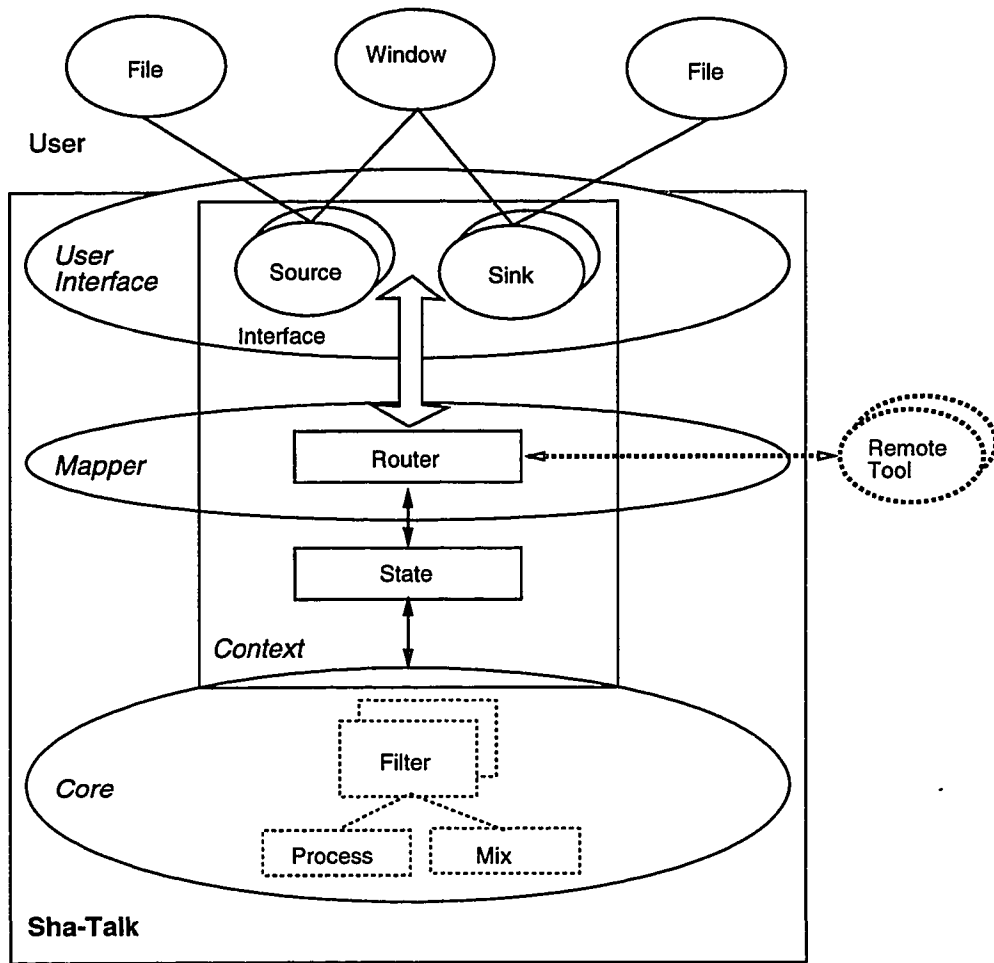
Figure B.1 High Level Architecture of Sha-Talk
