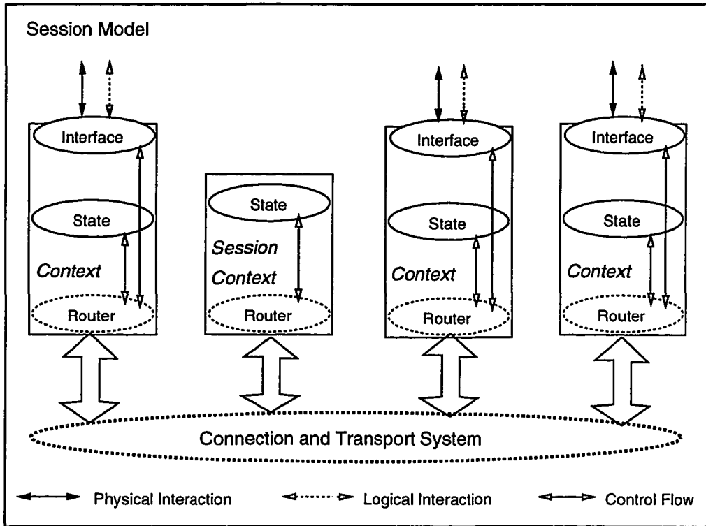
Figure 2.7 Session Model of Collaboration
