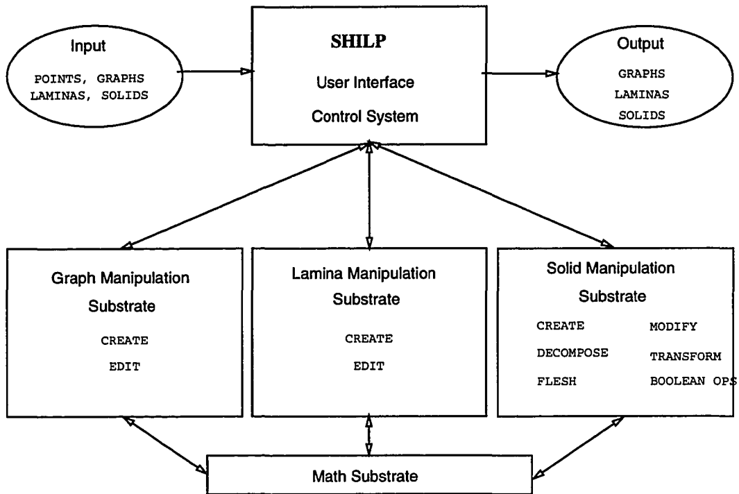
Figure C.1 Components of Shilp
