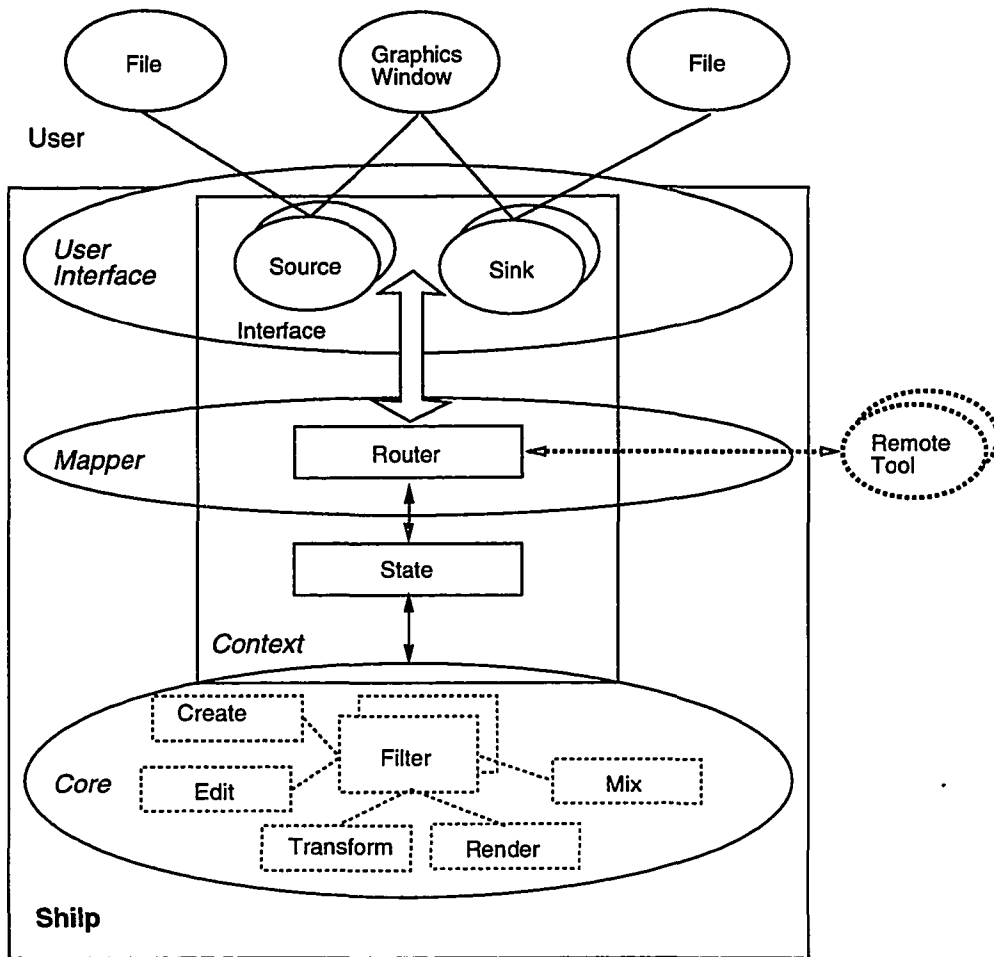
Figure C.3 Application Architecture of Shilp
