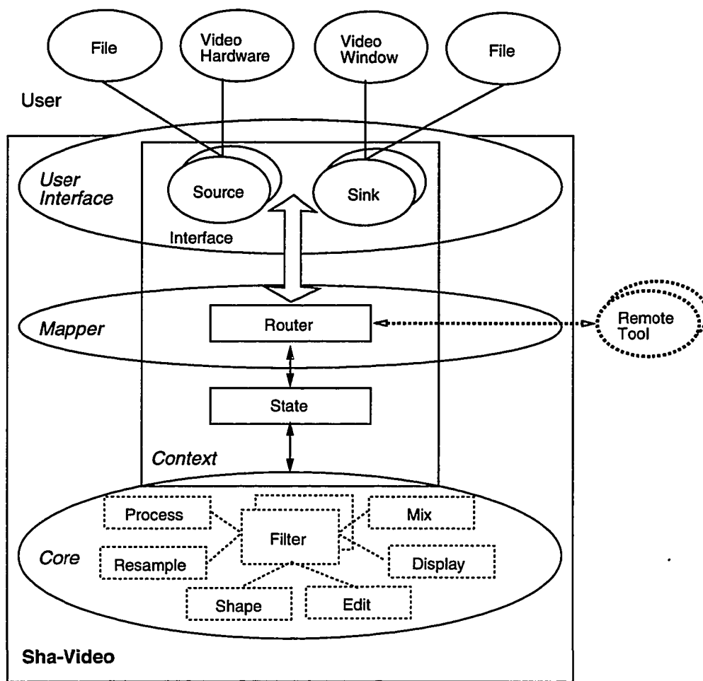
Figure B.6 High Level Architecture of Sha-Video
