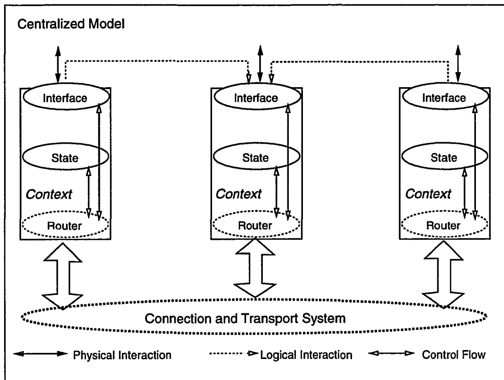
Figure 2.5 Centralized Collaboration Model
