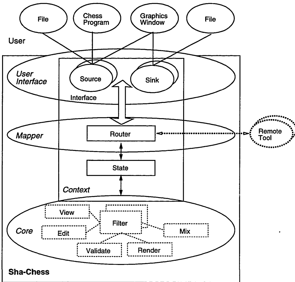
Figure D.2 High Level Architecture of Sha-Chess
