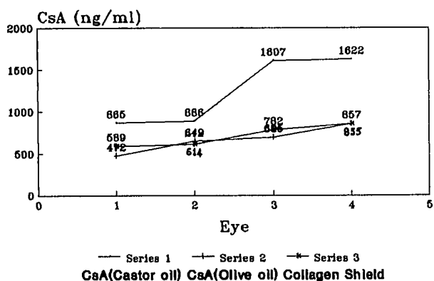
Figure 2 Cornea levels.
