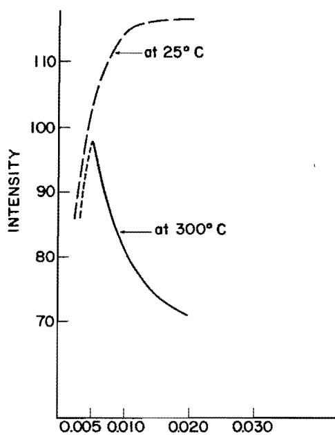
Figure 5. Emission intensity vs cerium content, measured at 25° C and 300° C. Excitation wavelength—436 nm.
