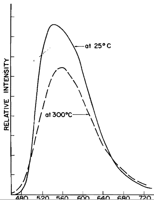
Figure 4. Emission curve: excitation wavelength—436 nanometers.
