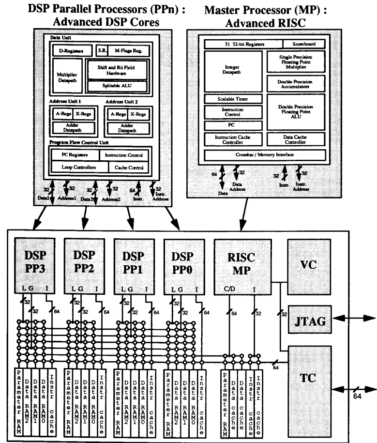
Figure 1: MVP Block Diagram: (A Single-Chip Parallel Processor)
