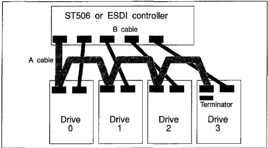
Figure 2.8 ST506 configuration.
