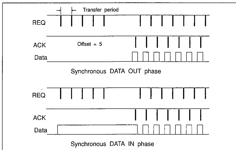
Figure 10.22 Synchronous data phases.
