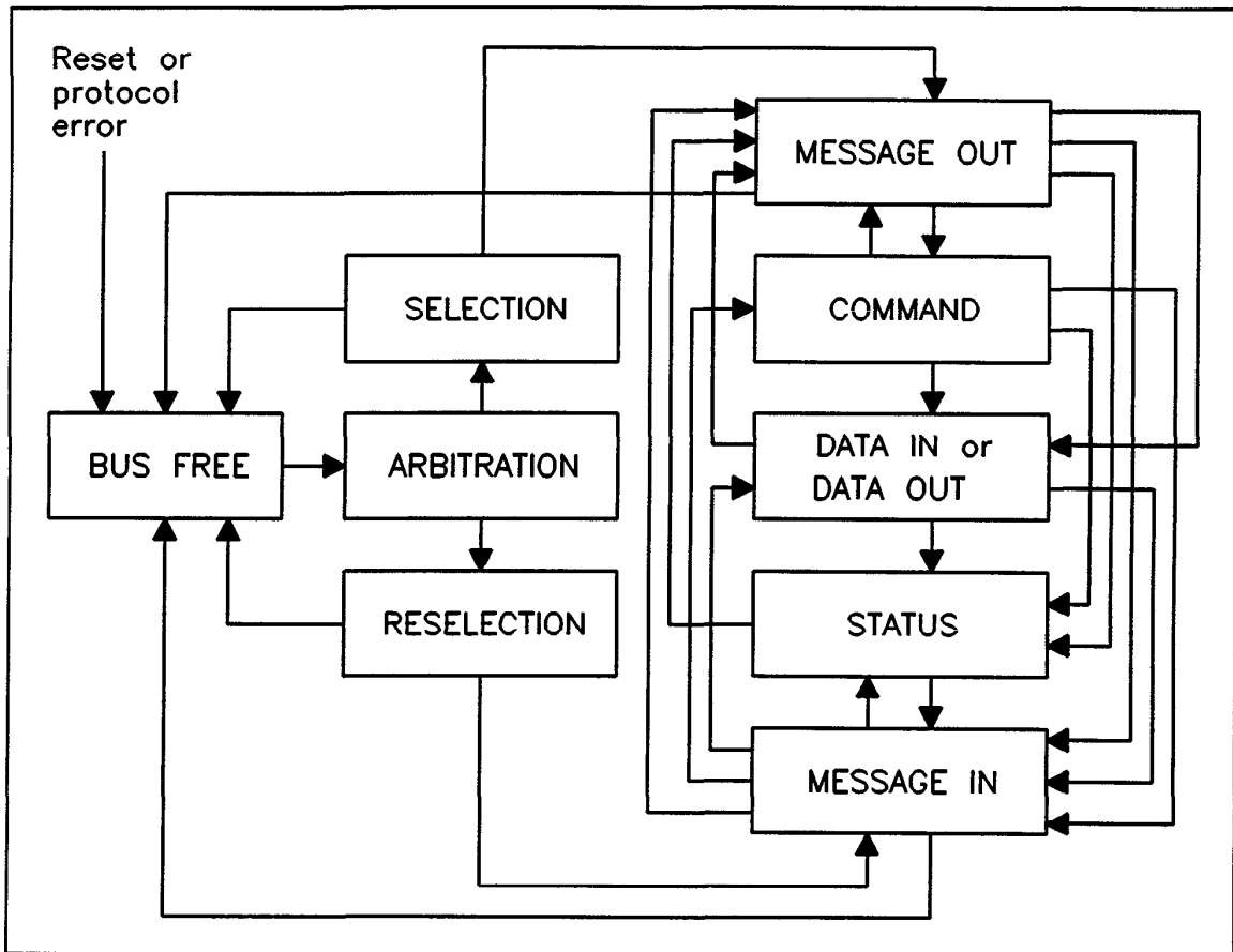
Figure 16 - Phase sequences
