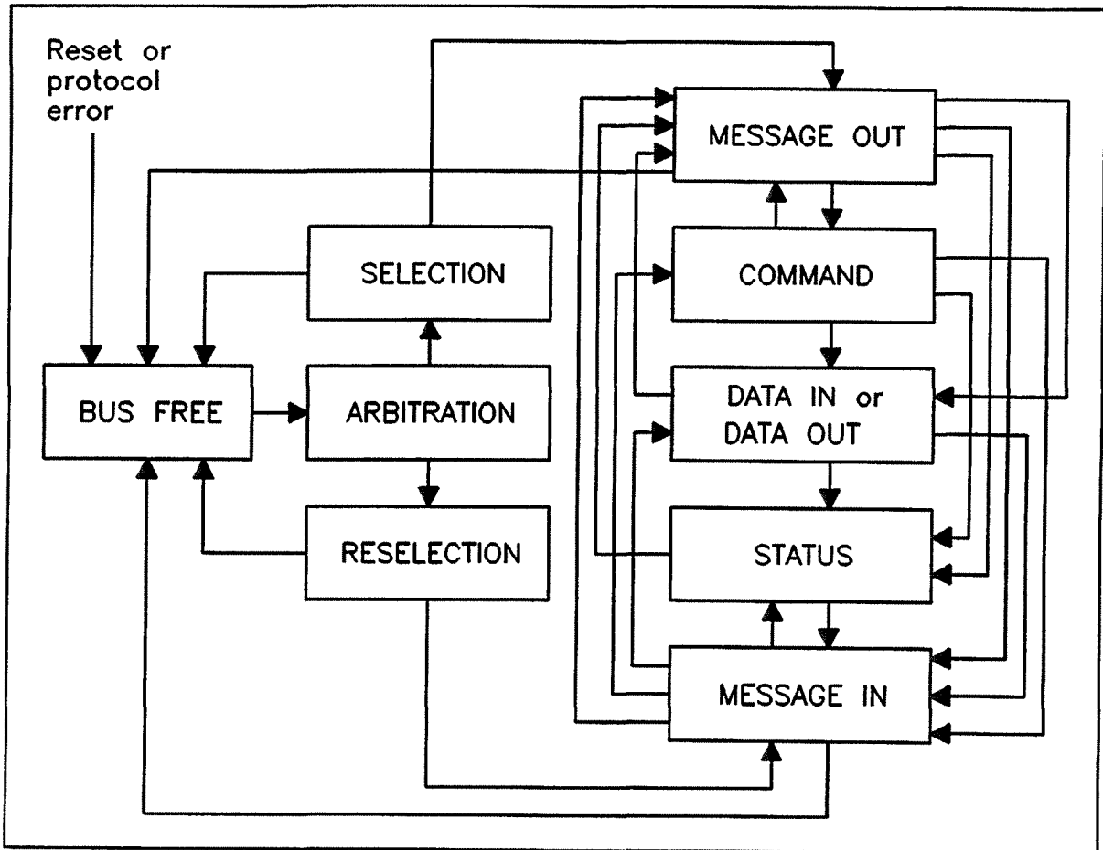
Figure 16 - Phase sequences
