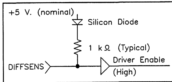
Figure 12 - Differential driver protection circuit
