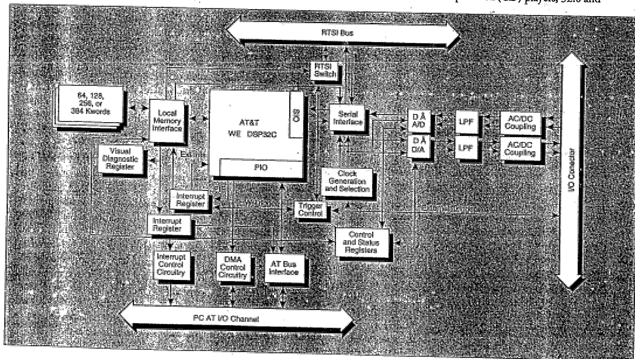
Figure 1. AT-DSP2200 Block Diagram
