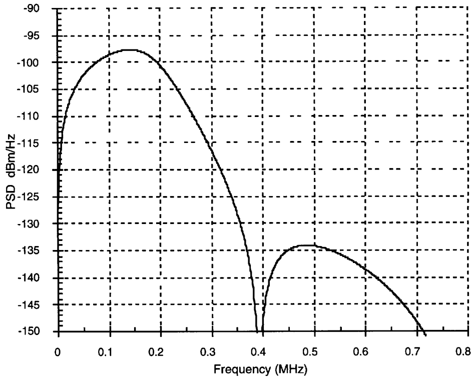
Figure B.2 – 10-disturber HDSL NEXT
