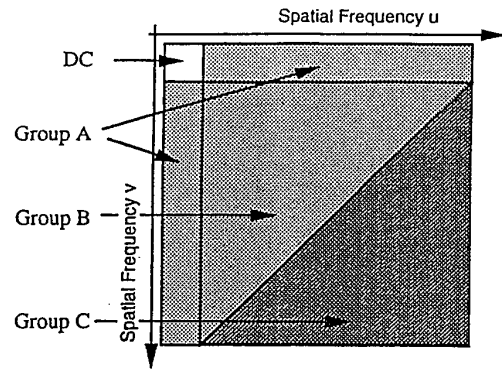
Figure 6. Separated DCT coefficient matrix
