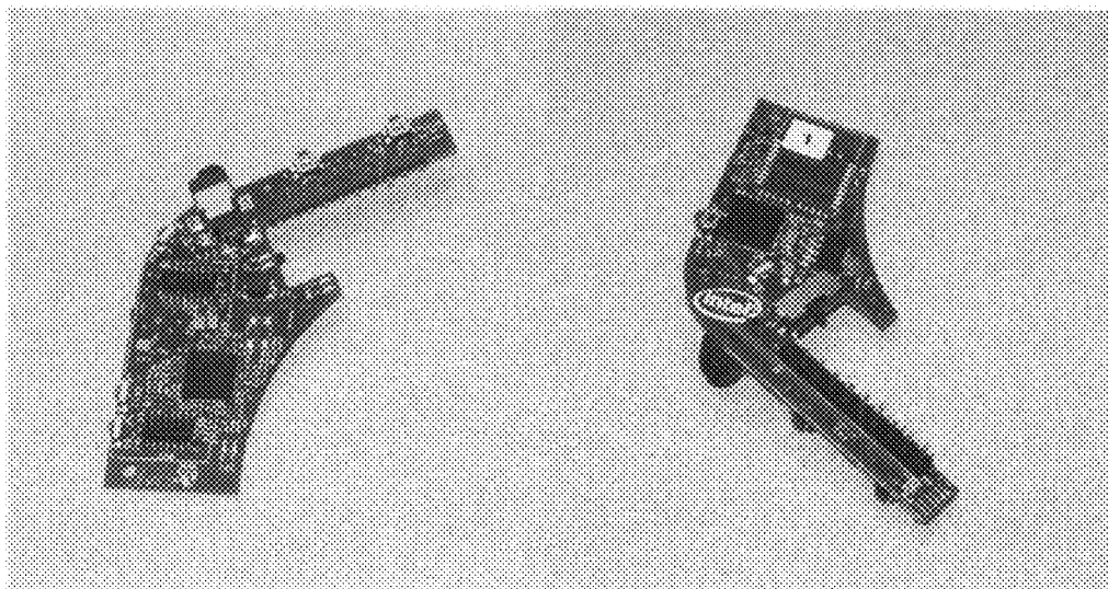
Figure 2 - Earpiece Circuit Board
