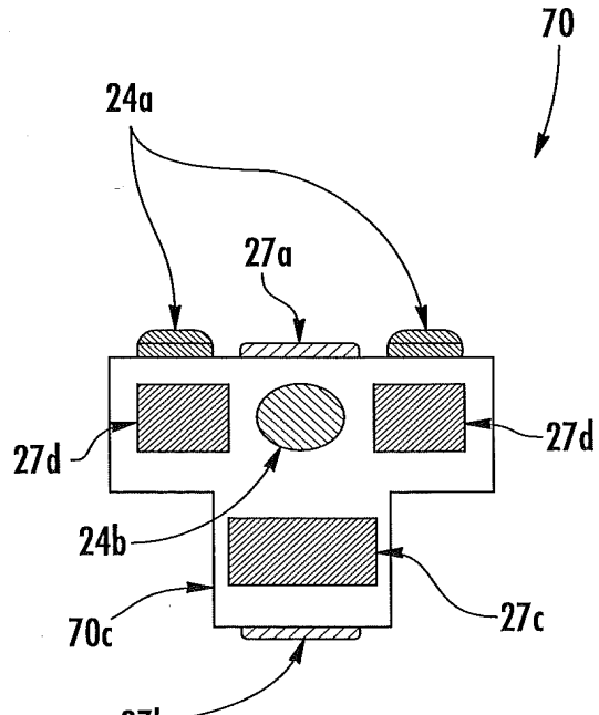
FACING EARBUD FIG. 12B
