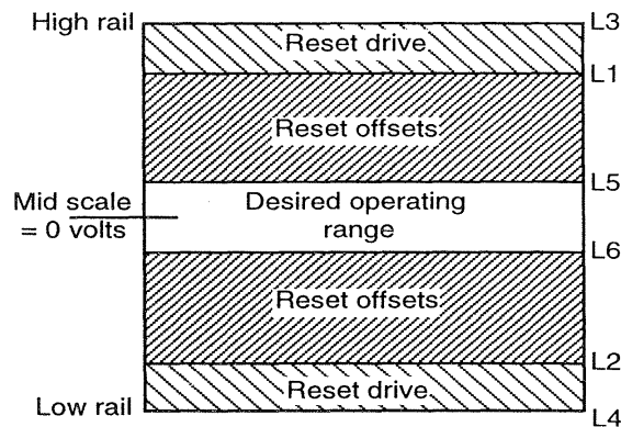
Figure 9.5 A graphical representation of the possible ranges of digitized signal, showing the desired response of the I/O circuit and microcomputer at each of the various possible ranges (Cheung et al 1989).
