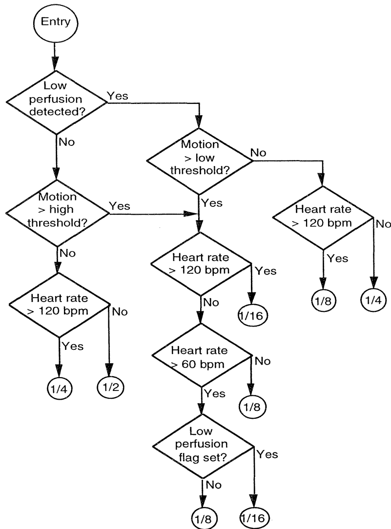
Figure 9.16. The weight determination algorithm (Conlon et al 1990).
