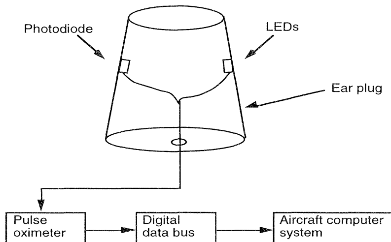
Figure 13.3 Modified pulse oximeter probe for use in the ear canal. In this version, a clay mold has been used to produce the ear plug with the LEDs and photodiode pressed into the sides (adapted from Tripp 1993).
