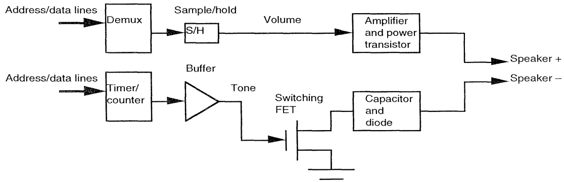
Figure 8.16 Speaker driver block diagram (adapted from Nellcor N-200 ® (Nellcor 1989)).
