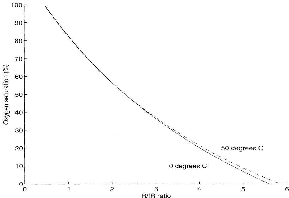
Figure 11.7 The calibration curves from a theoretical model show a shift from 0 °C to 50 °C.
