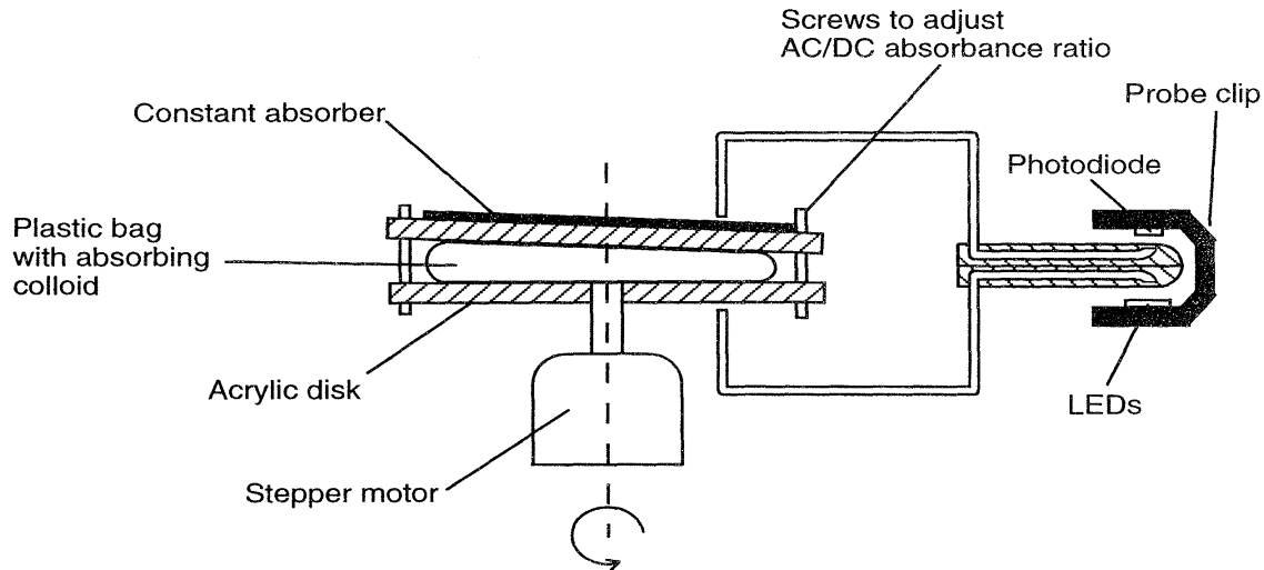
Figure 10.9 Leuthner’s (1994) colored colloid disk system.
