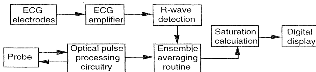
Figure 9.8. Block diagram illustrating the ECG processing components, its subcomponents and their relationship in an oximeter.
