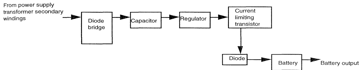
Figure 8.14 Battery charger block diagram (adapted from Nellcor N-200 ® (Nellcor 1989)).
