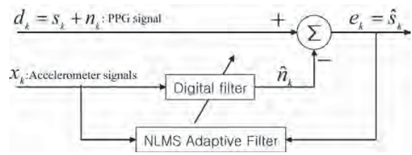
Fig. 3. Block diagram of the active noise cancellation algorithm
