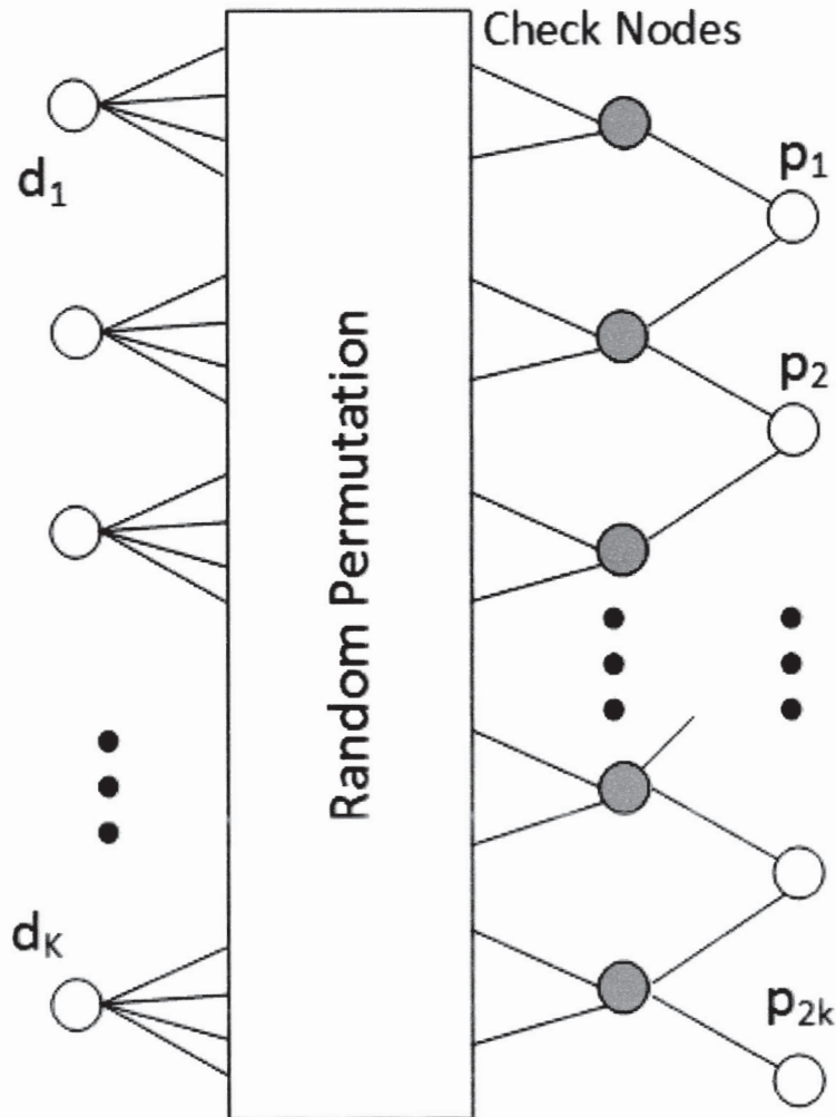
Tanner graph for Ping (with t=4 , k=30,000 , and n=90,000 )
